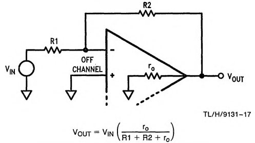
FIGURE 11. Inverting Gain Channel Feedthrough
