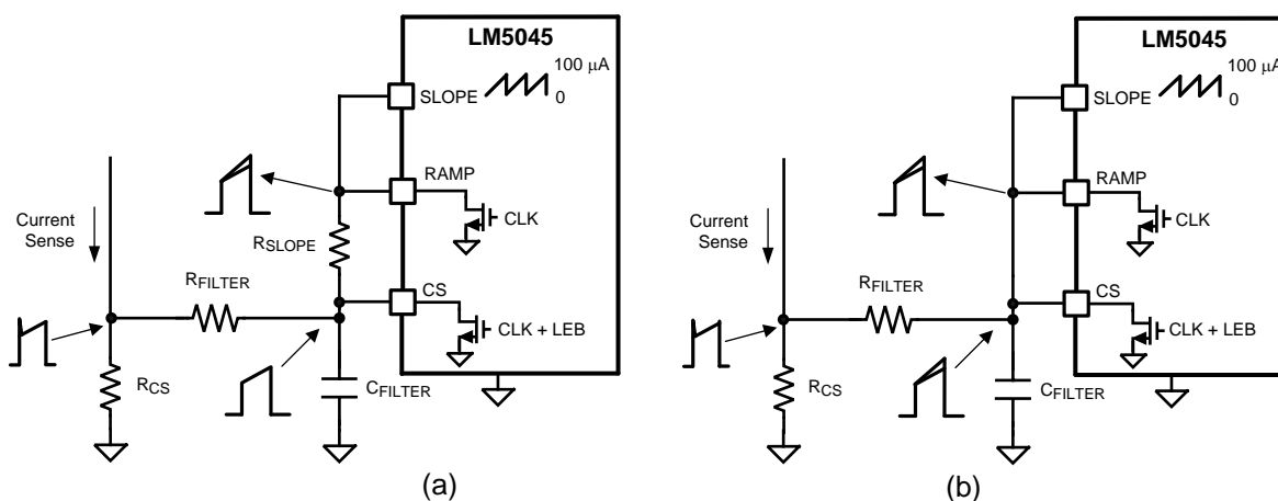
Figure 13. Slope Compensation Configuration
