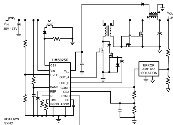
Figure 1. Simplified Active Clamp Forward Power Converter
