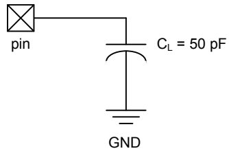
Figure 25-1. Load Conditions
