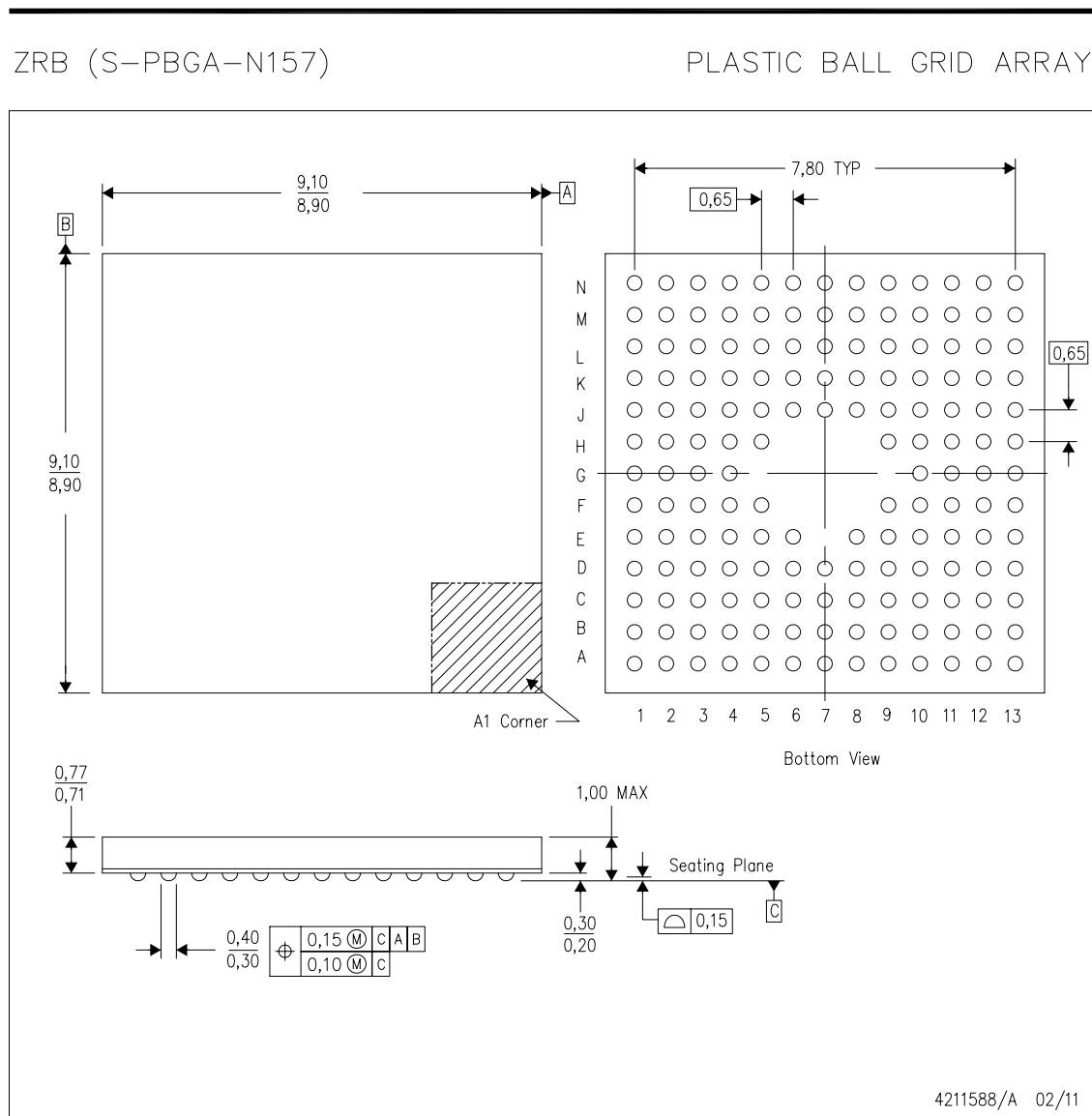
Figure B-1. Stellaris® LM4F232H5BB 157-Ball BGA Package Dimensions
