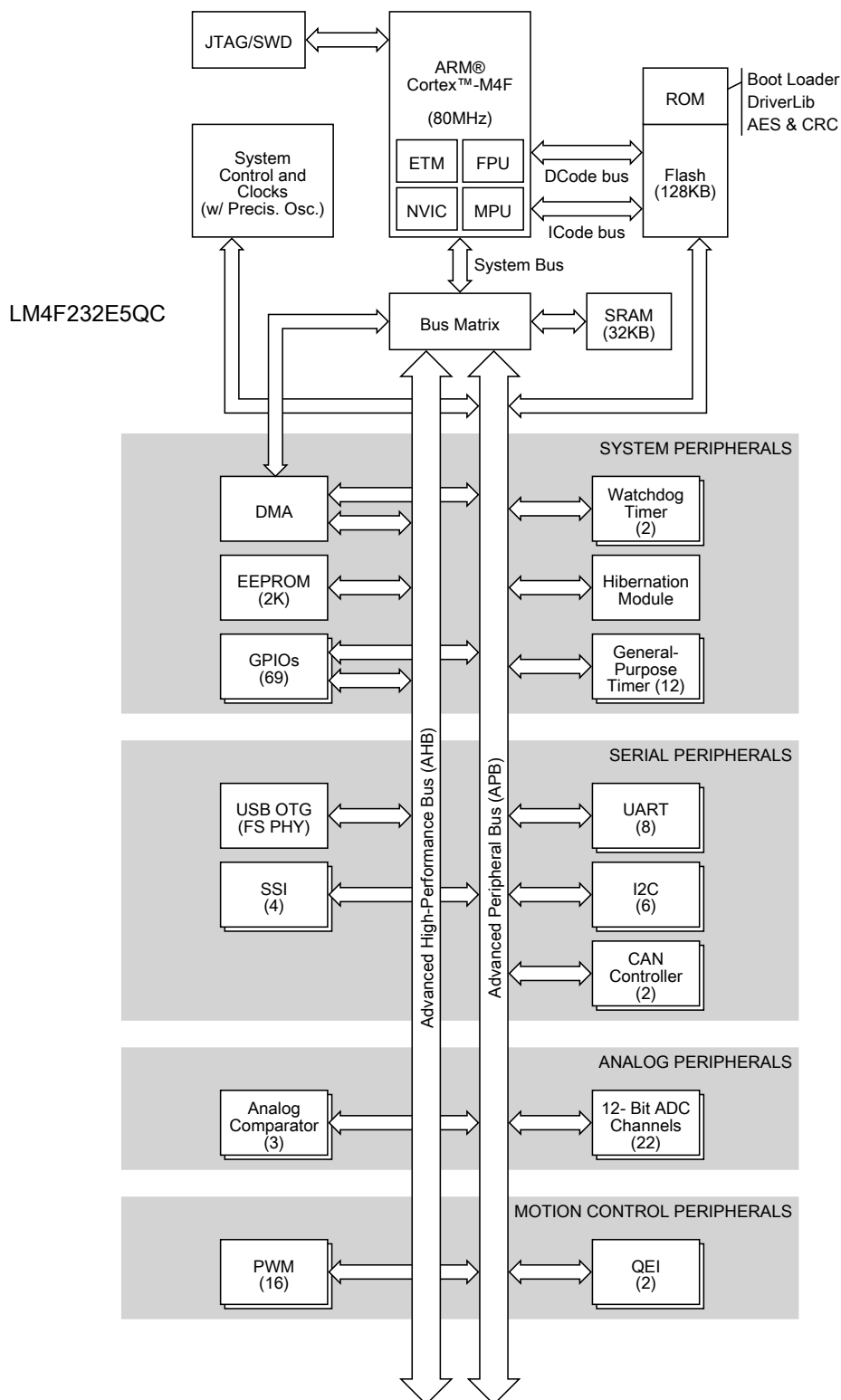
Figure 1-2. Stellaris LM4F232E5QC Microcontroller High-Level Block Diagram
