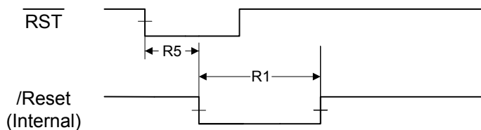
Figure 25-5. Software Reset Timing
