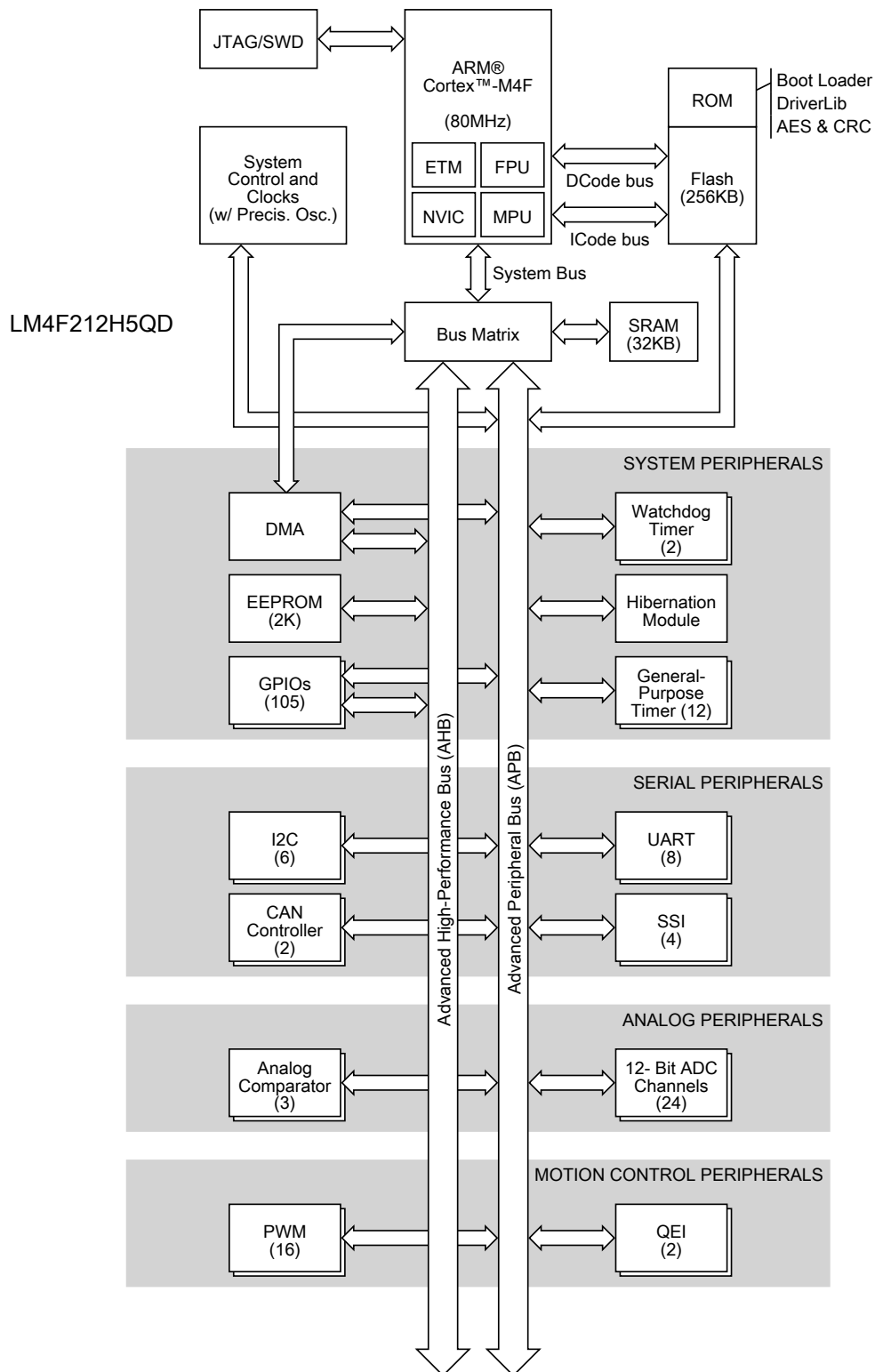
Figure 1-2. Stellaris LM4F212H5QD Microcontroller High-Level Block Diagram
