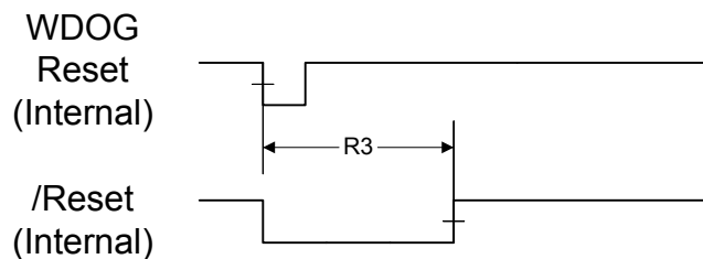
Figure 24-6. Watchdog Reset Timing
