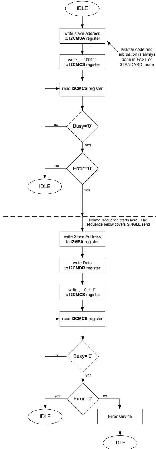
Figure 16-14. High Speed Mode Master Transmit
