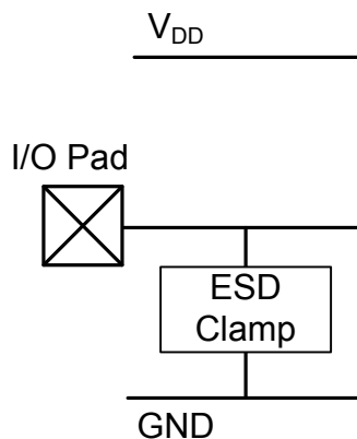
Figure 24-9. ESD Protection on Fail-Safe Pins
