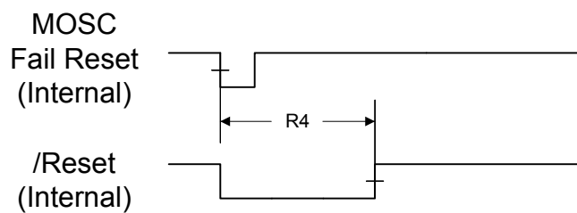
Figure 24-7. MOSC Failure Reset Timing
