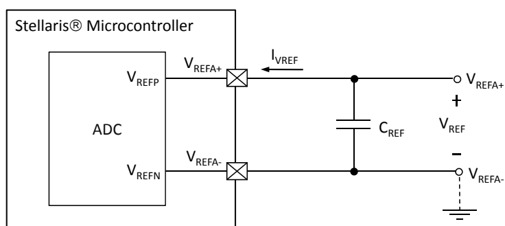
Figure 24-12. ADC Input Equivalency Diagram
