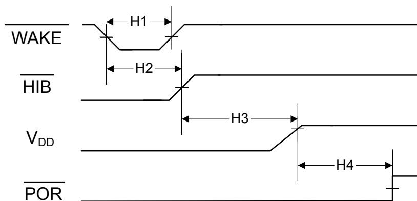
Figure 24-8. Hibernation Module Timing
