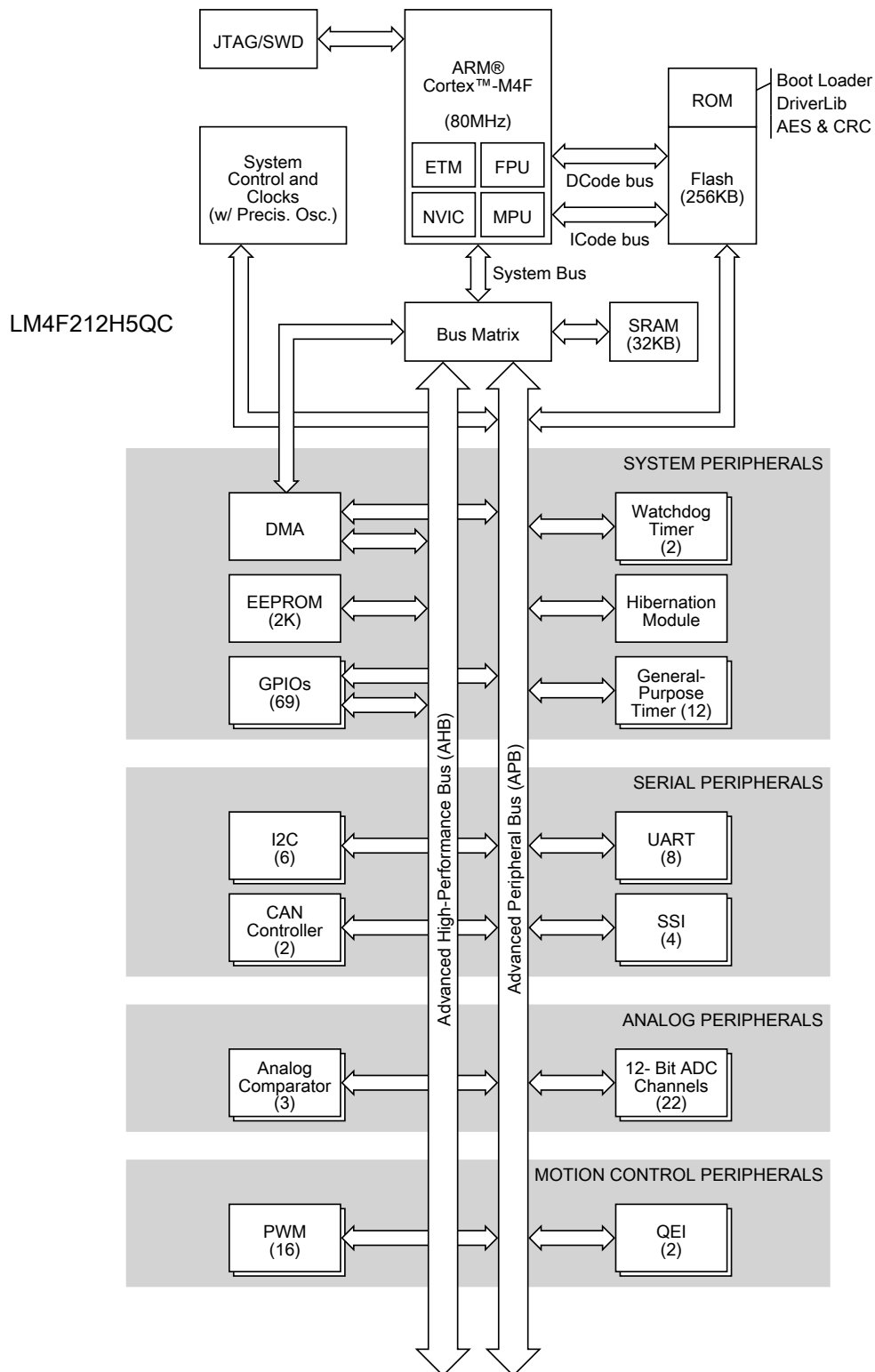
Figure 1-2. Stellaris LM4F212H5QC Microcontroller High-Level Block Diagram
