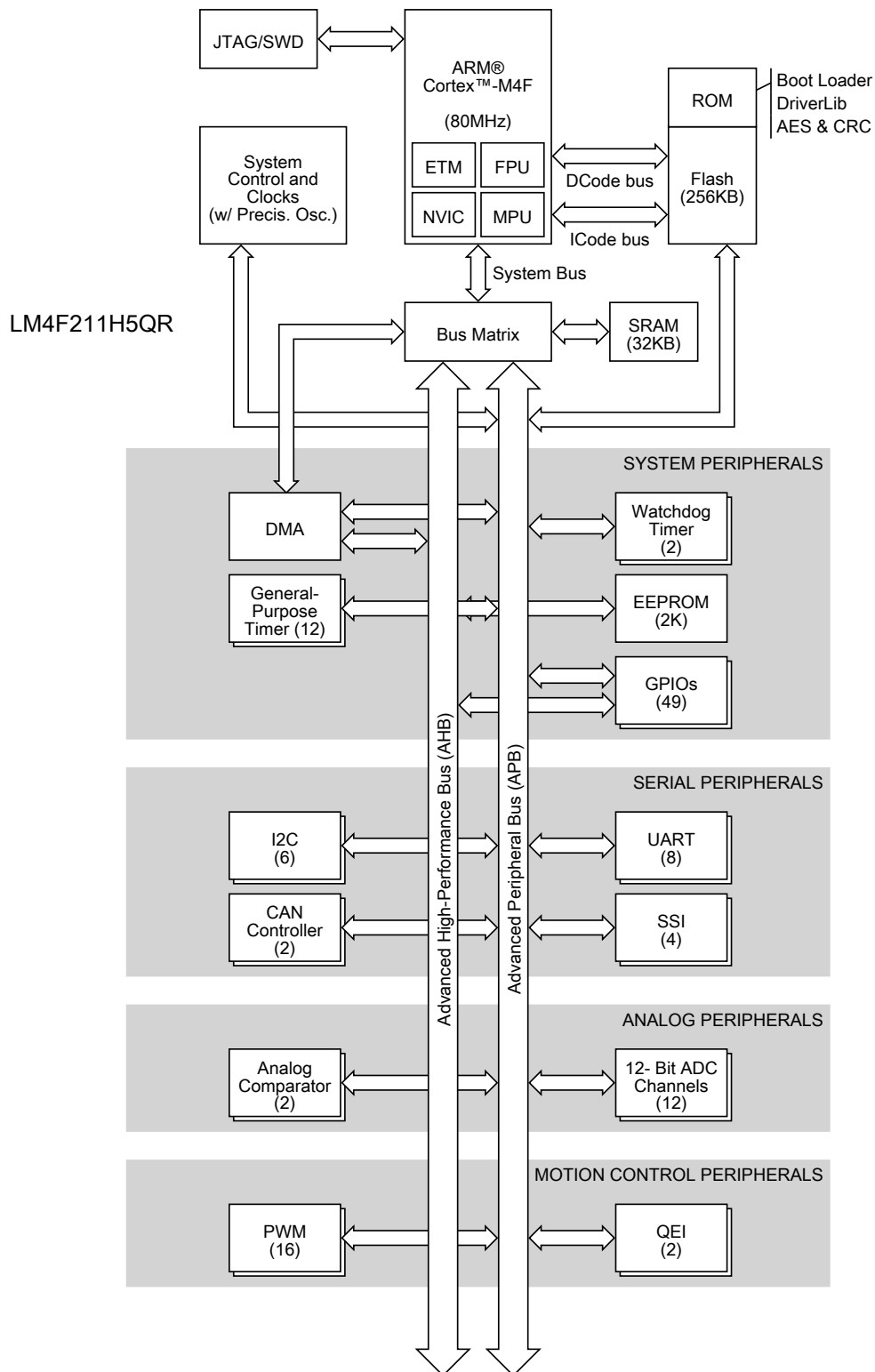
Figure 1-2. Stellaris LM4F211H5QR Microcontroller High-Level Block Diagram
