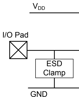
Figure 23-8. ESD Protection on Fail-Safe Pins
