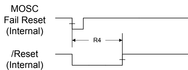
Figure 23-7. MOSC Failure Reset Timing
