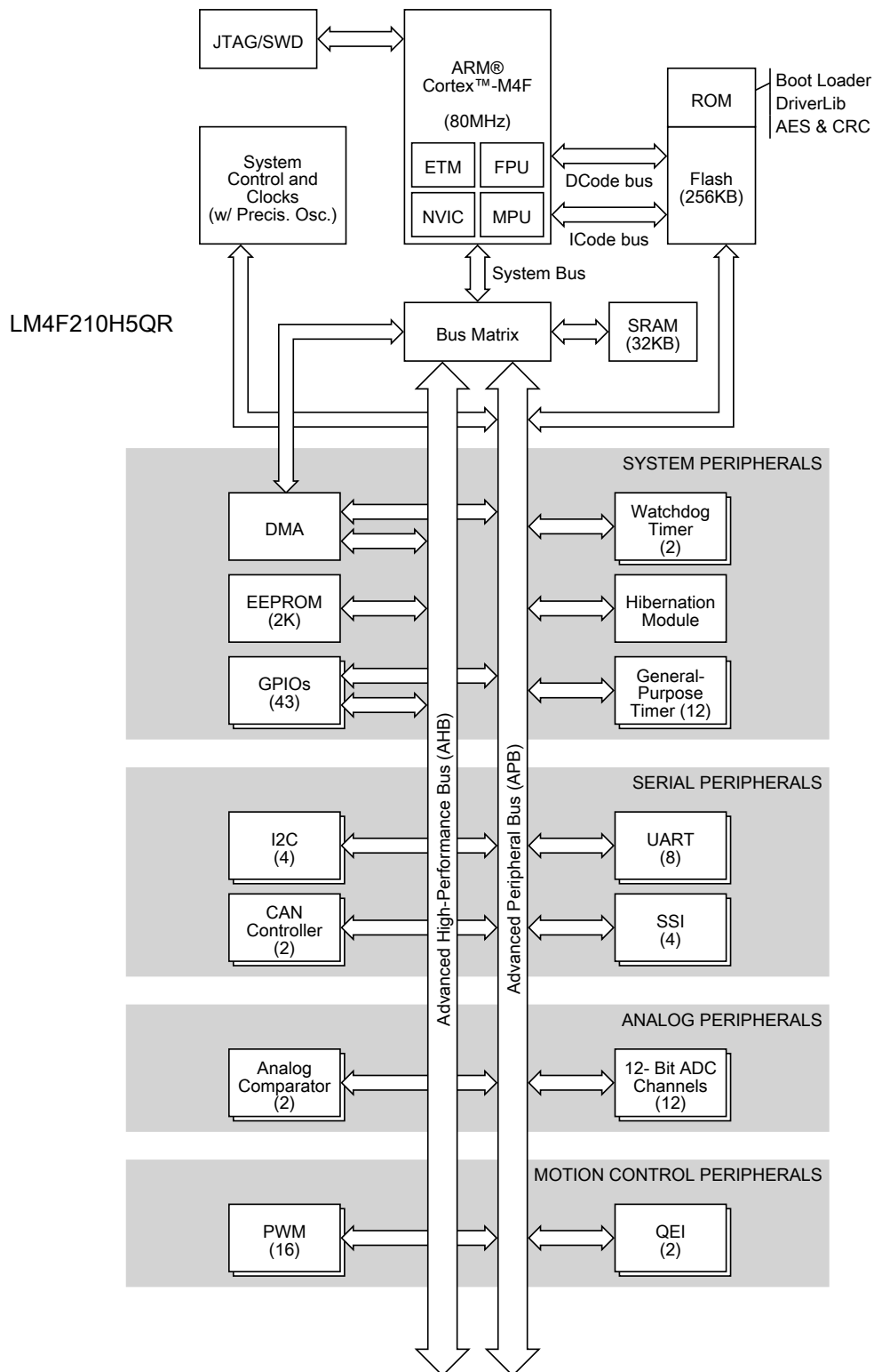
Figure 1-2. Stellaris LM4F210H5QR Microcontroller High-Level Block Diagram
