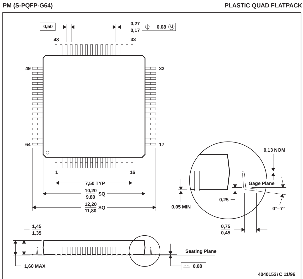
Figure B-1. Stellaris® LM4F210E5QR 64-Pin LQFP Package
