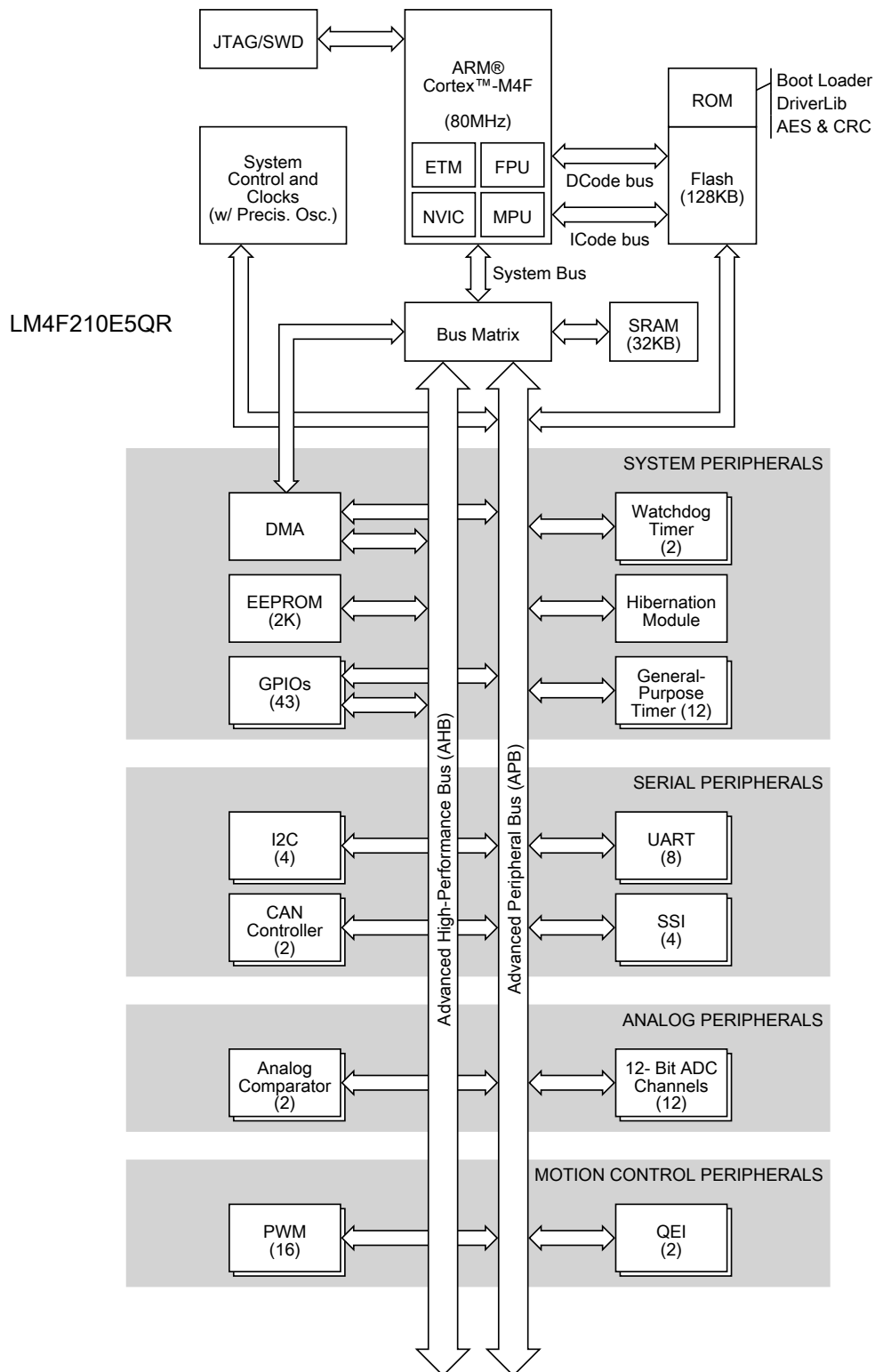
Figure 1-2. Stellaris LM4F210E5QR Microcontroller High-Level Block Diagram
