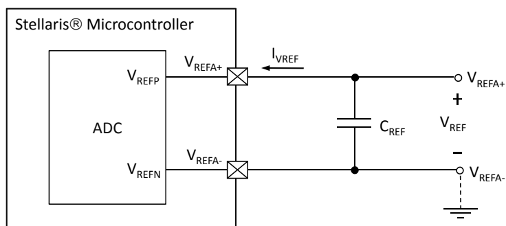
Figure 23-12. ADC Input Equivalency Diagram
