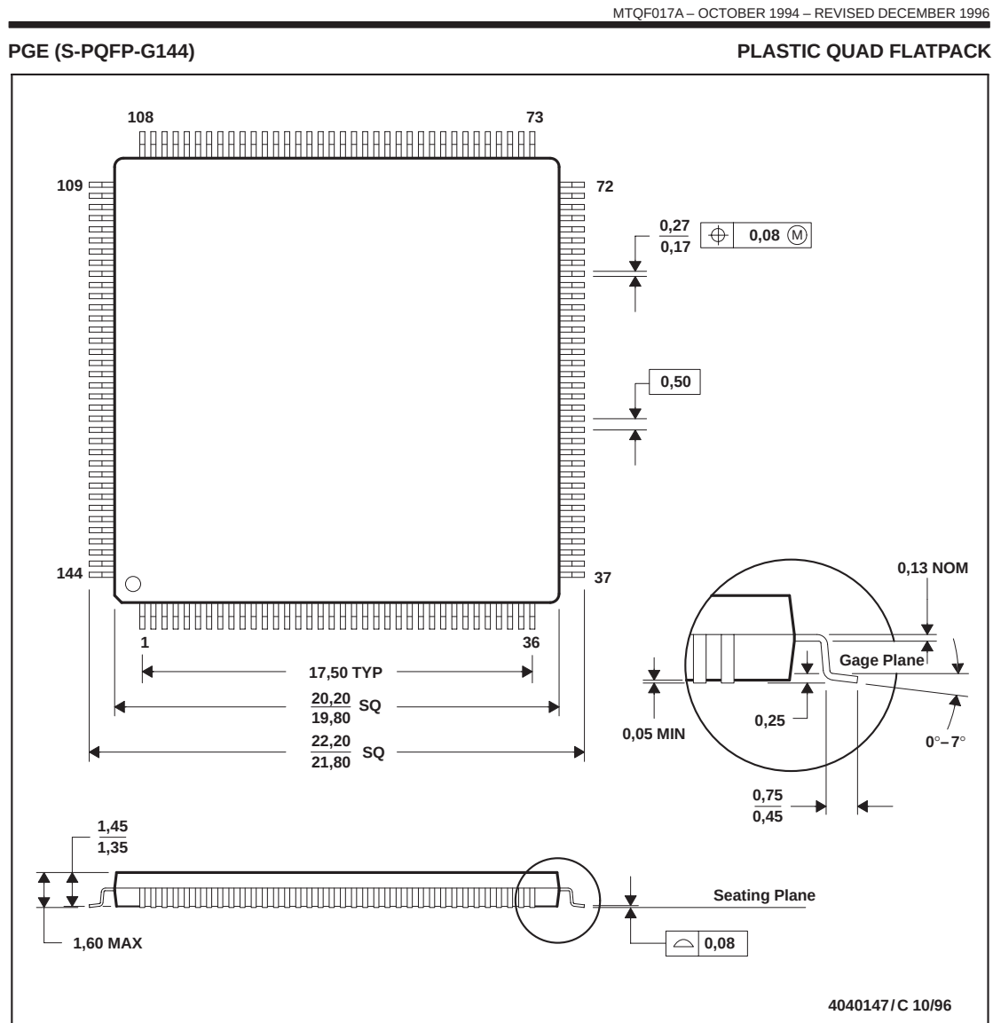
Figure B-1. Stellaris® LM4F122H5QD 144-Pin LQFP Package Dimensions
