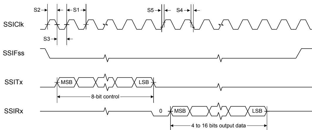
Figure 23-14. SSI Timing for MICROWIRE Frame Format (FRF=10), Single Transfer
