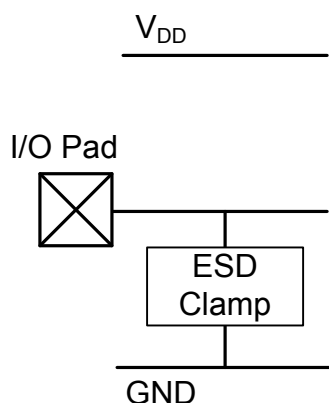
Figure 23-9. ESD Protection on Fail-Safe Pins
