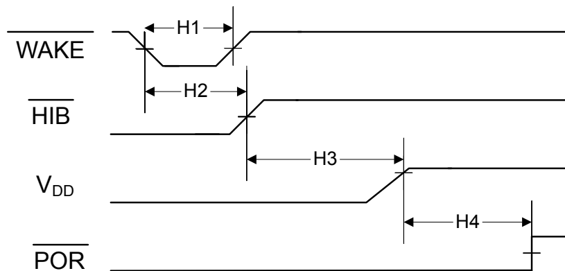
Figure 23-8. Hibernation Module Timing
