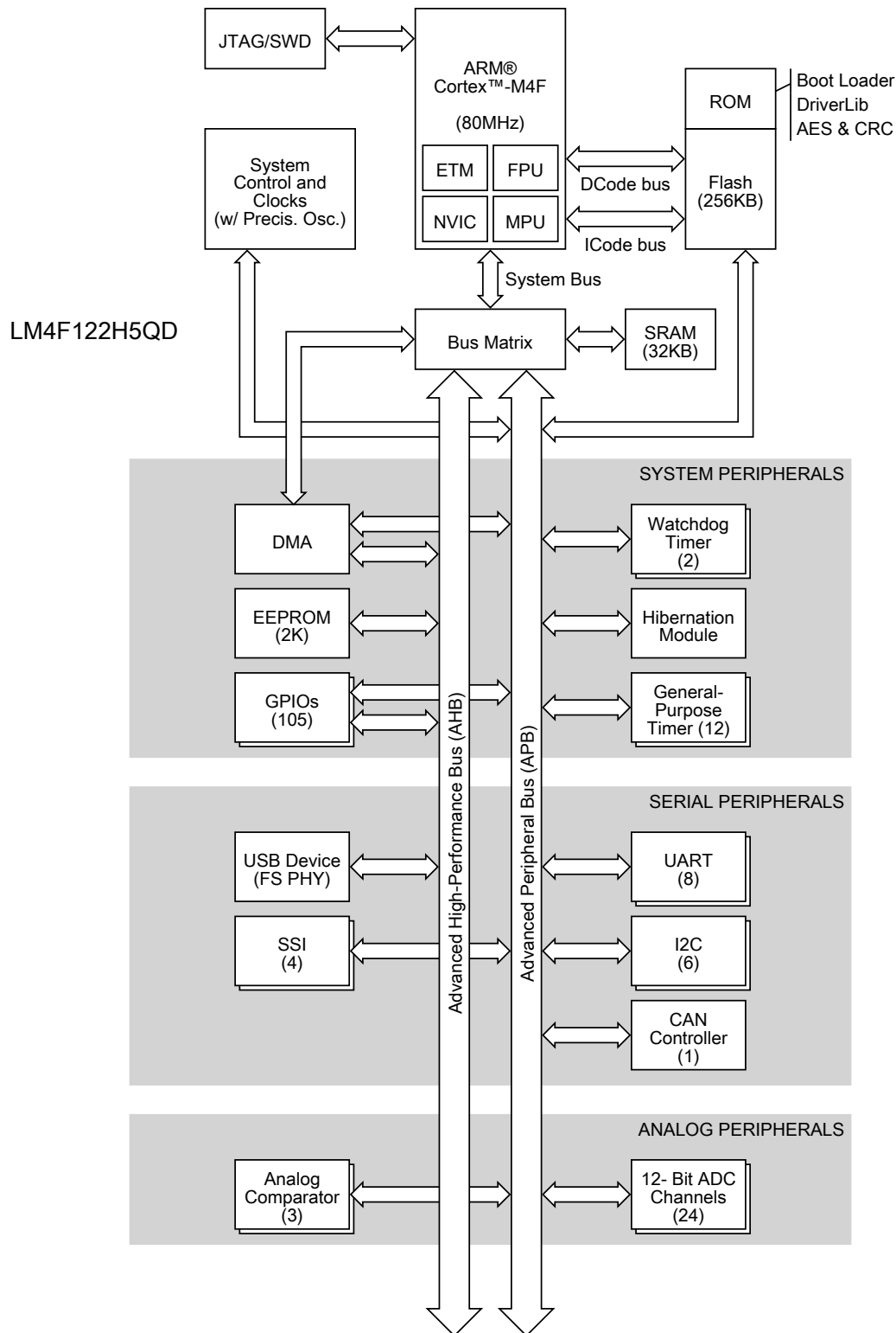
Figure 1-2. Stellaris LM4F122H5QD Microcontroller High-Level Block Diagram
