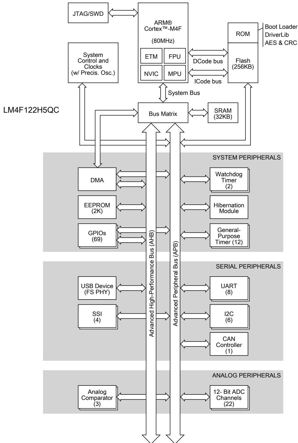
Figure 1-2. Stellaris LM4F122H5QC Microcontroller High-Level Block Diagram
