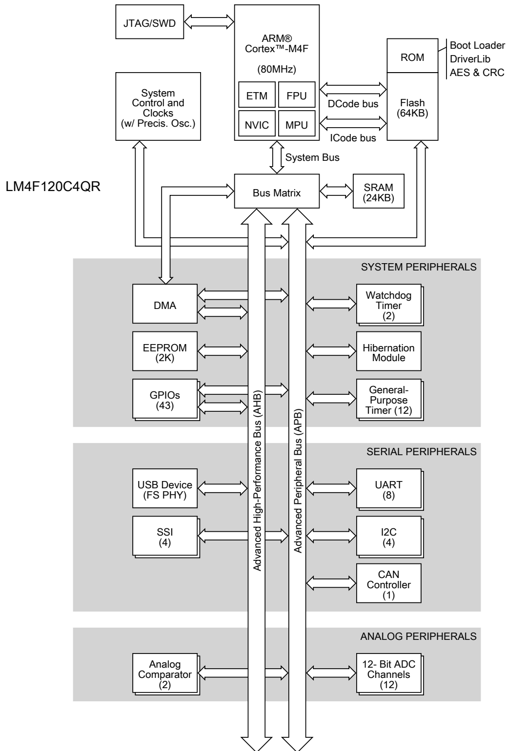
Figure 1-2. Stellaris LM4F120C4QR Microcontroller High-Level Block Diagram
