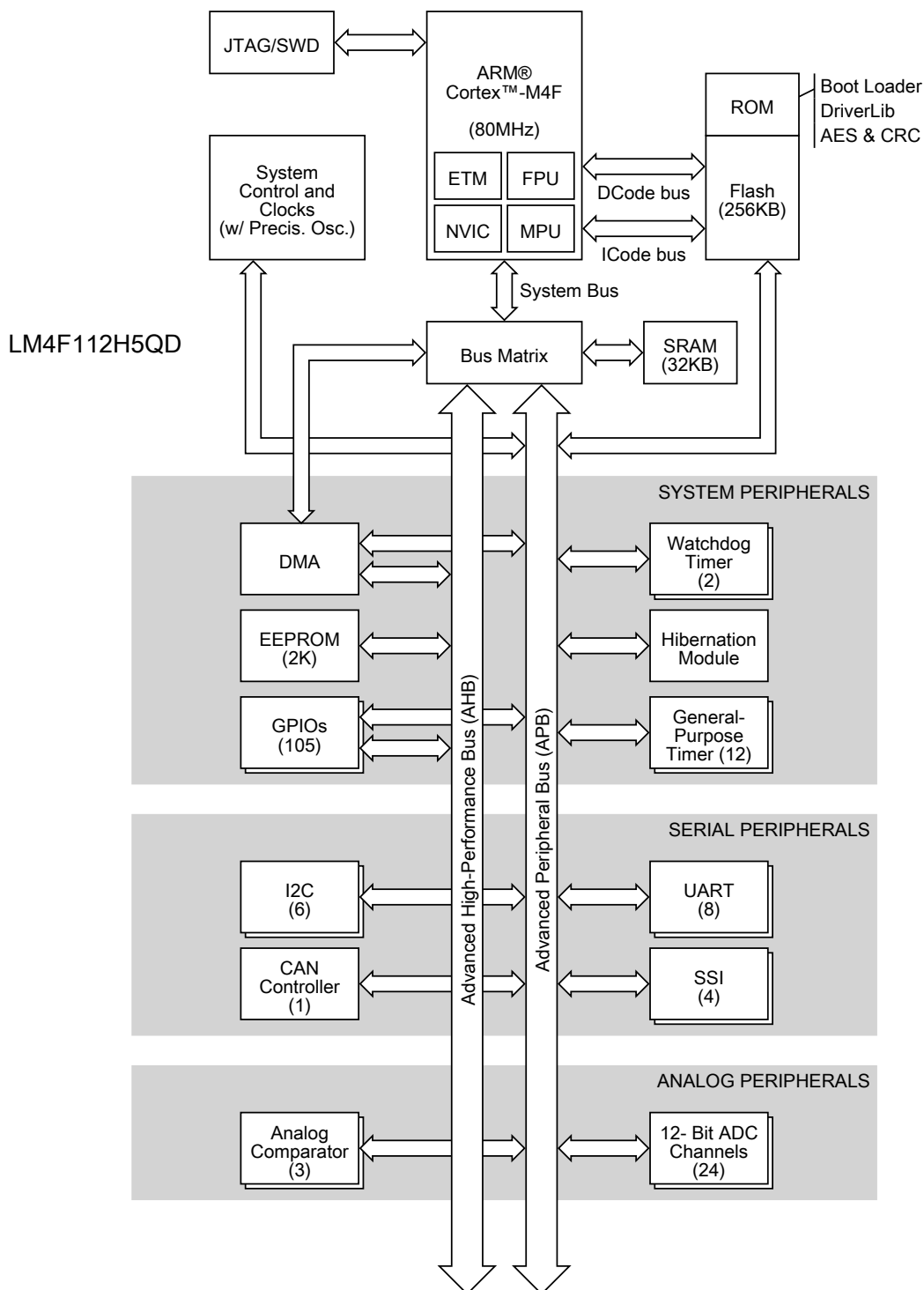
Figure 1-2. Stellaris LM4F112H5QD Microcontroller High-Level Block Diagram
