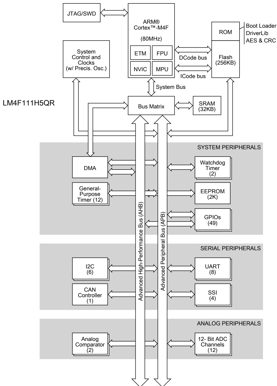
Figure 1-2. Stellaris LM4F111H5QR Microcontroller High-Level Block Diagram
