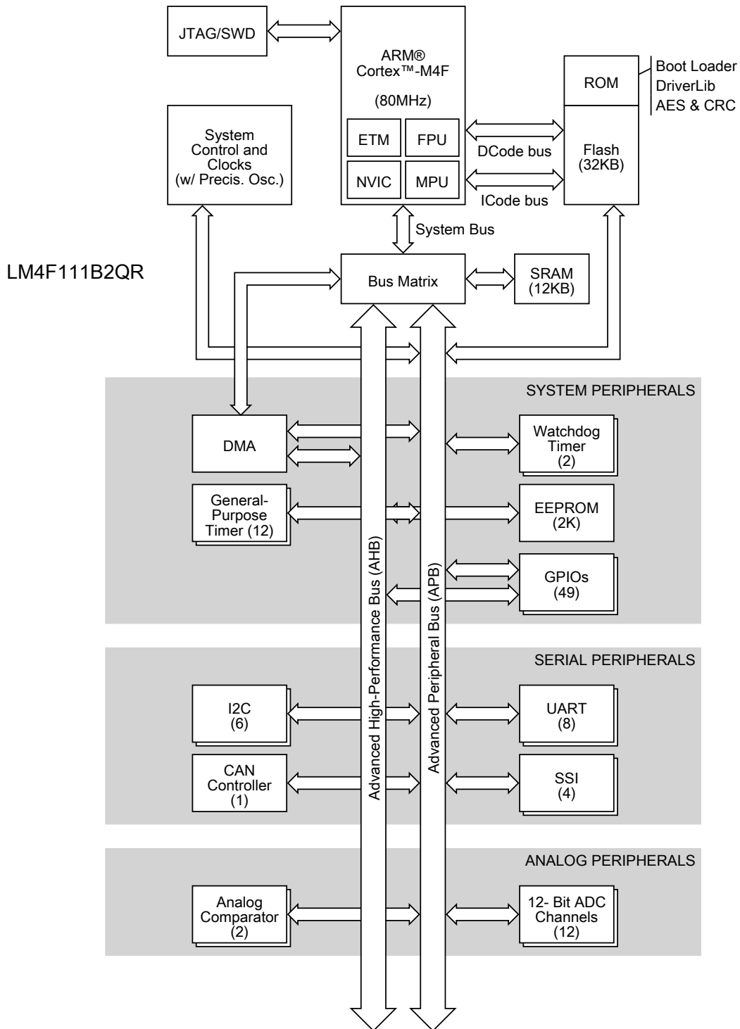
Figure 1-2. Stellaris LM4F111B2QR Microcontroller High-Level Block Diagram
