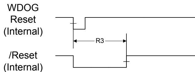
Figure 21-6. Watchdog Reset Timing
