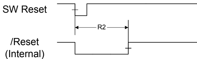
Figure 21-5. Software Reset Timing
