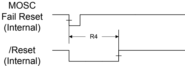
Figure 21-7. MOSC Failure Reset Timing
