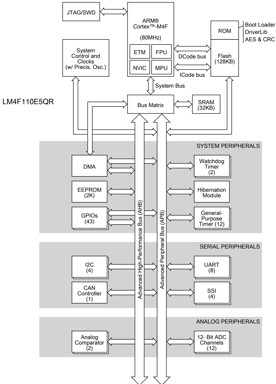
Figure 1-2. Stellaris LM4F110E5QR Microcontroller High-Level Block Diagram
