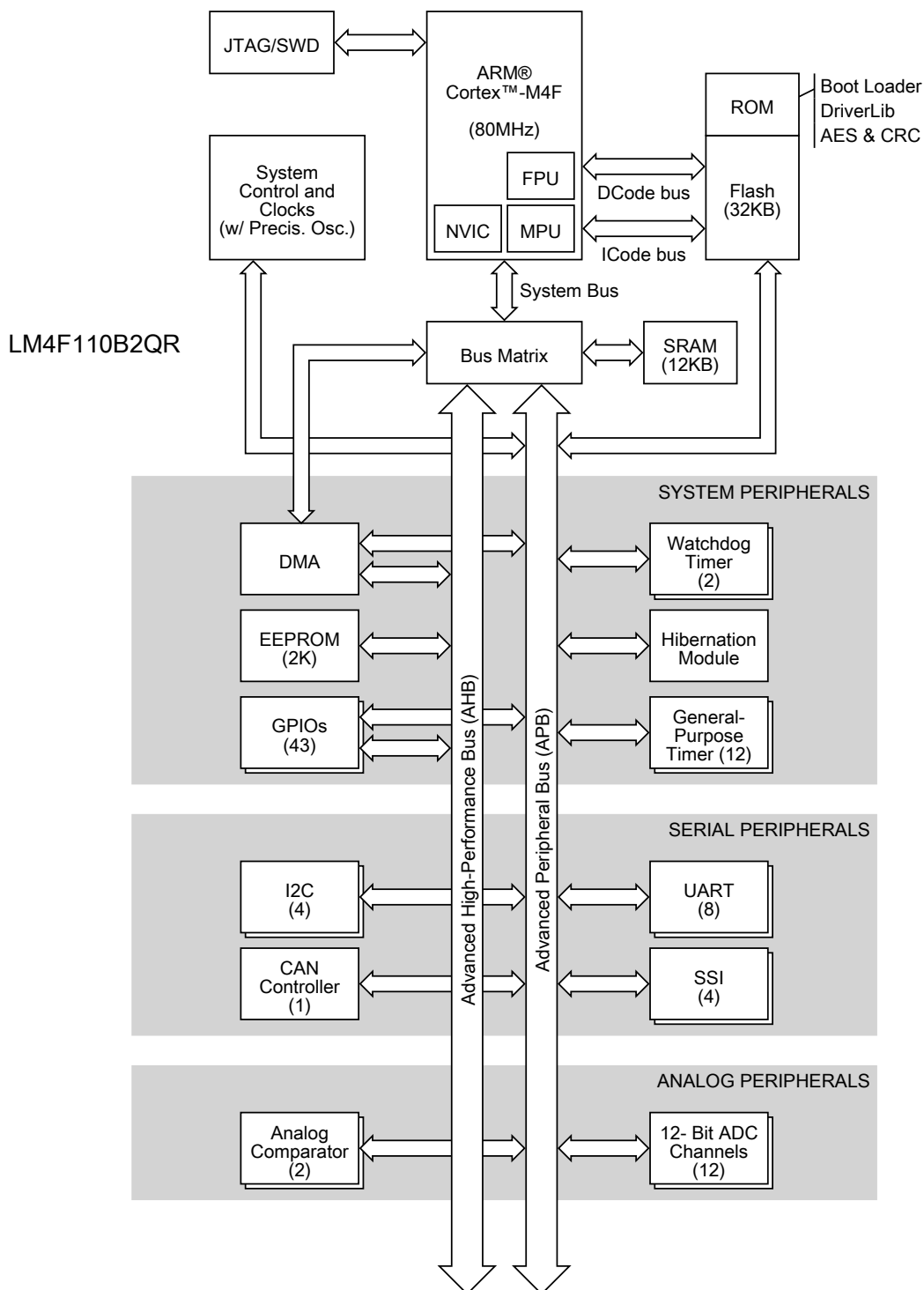
Figure 1-2. Stellaris LM4F110B2QR Microcontroller High-Level Block Diagram
