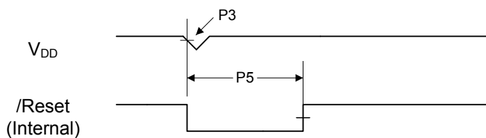
Figure 22-5. Brown-Out Reset Timing
