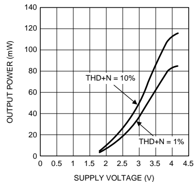
Output Power vs Supply Voltage R_L = 16\Omega, f = 1kHz, \text{two channels}
