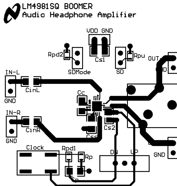
Figure 4. Top Layer
