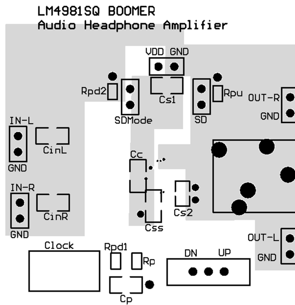
Figure 5. Mid Layer 1
