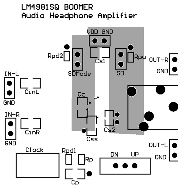
Figure 6. Mid Layer 2
