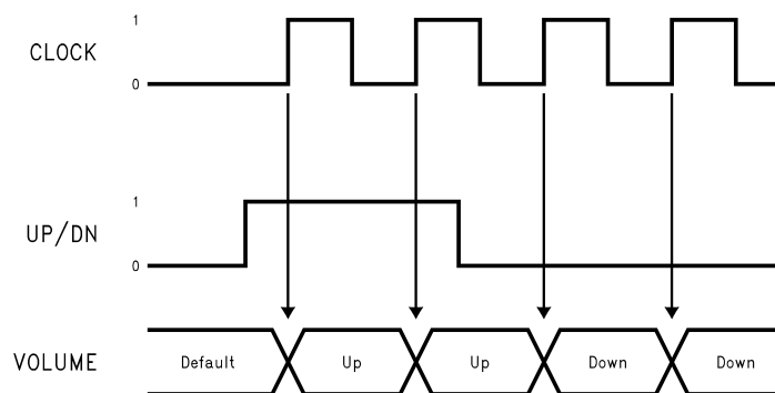
Figure 2. Timing Diagram
