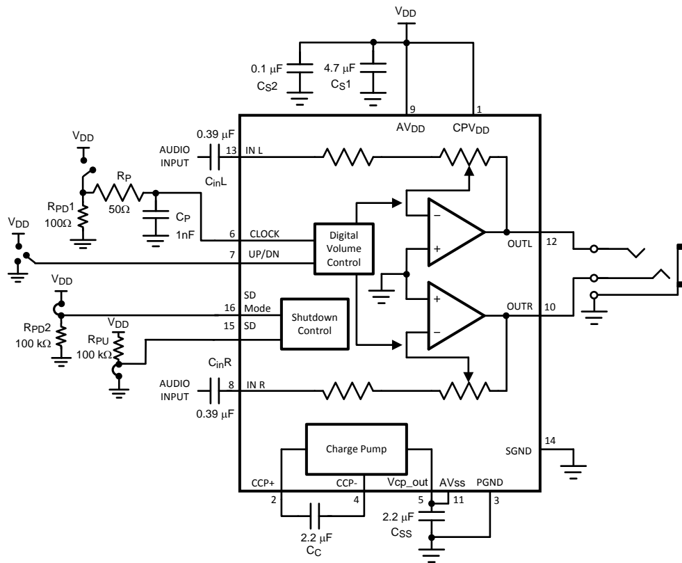
Figure 3. Demo Board Schematic
