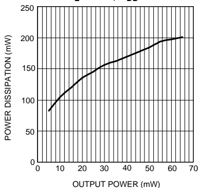
Power Dissipation vs Output Power R_L = 32\Omega , V_{DD} = 3\text{V}
