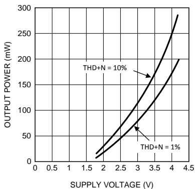
Output Power vs Supply Voltage R_L = 16\Omega, f = 1kHz, \text{one channel}
