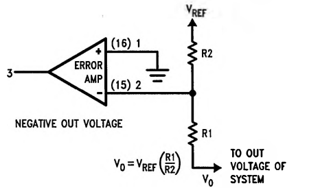
FIGURE 7. Error Amplifier Sensing Techniques
