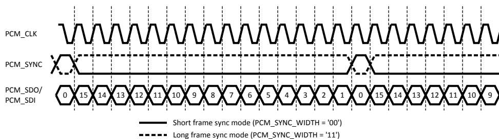
Figure 22. PCM Serial Data Format (16 bit Slave Example)
