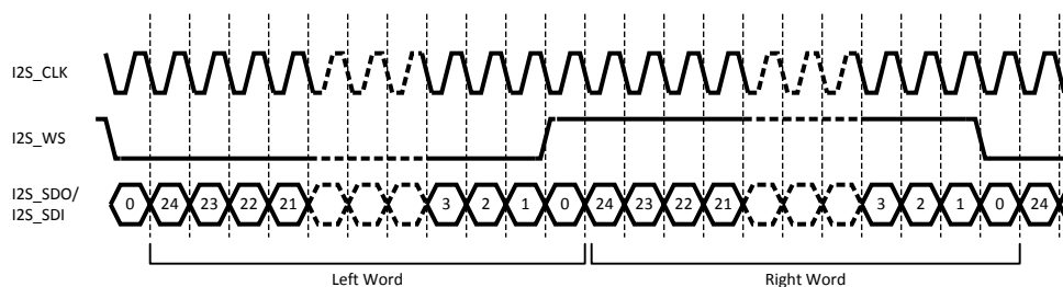
Figure 20. I 2 S Serial Data Format (Default Mode)
