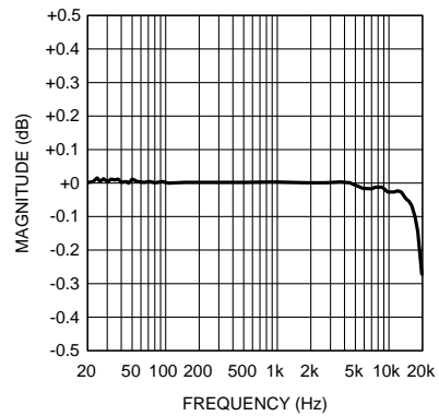
Stereo DAC Frequency Response Zoom f_s = 48kHz
