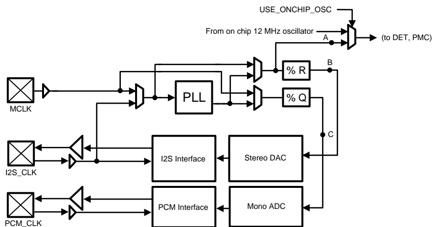
Figure 14. LM49370 Clock Network
