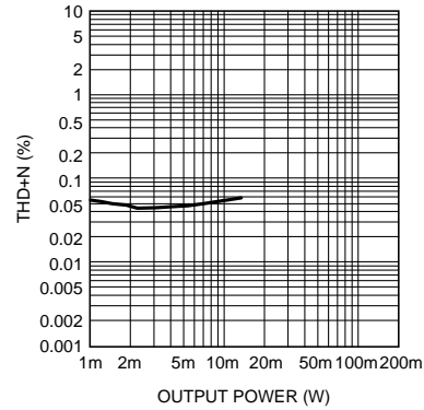
Headphone THD+N vs Output Power AV_{DD} = 3.3V, SE, 0dB DAC f_{OUT} = 1kHz, 32\Omega
