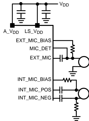
Figure 27. Schematic Option for ECM Microphones
