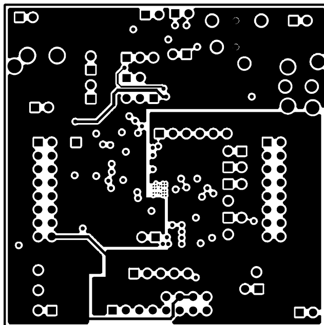
Figure 30. Mid Layer 1
