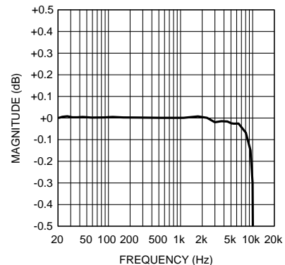
Stereo DAC Frequency Response Zoom f_S = 24kHz
