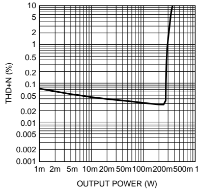
Headphone THD+N vs Output Power AV_{DD} = 5V, OCL\ 1.2V, 0dB\ DAC f_{OUT} = 1kHz, 16\Omega
