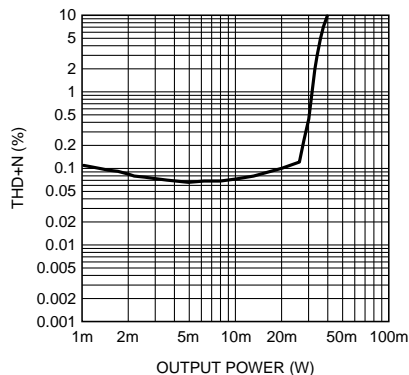
Headphone THD+N vs Output Power AV_{DD} = 3.3V , OCL 1.5V, 12dB DAC f_{OUT} = 1kHz , 32Ω
