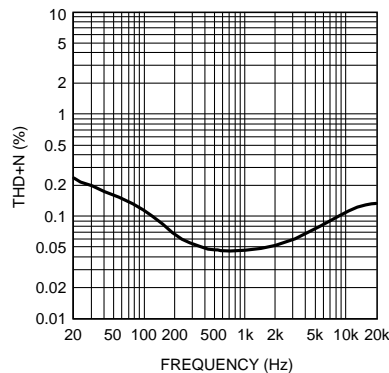
Loudspeaker THD+N vs Frequency AV_{DD} = 3.3V, P_{OUT} = 400mW 15\mu H + 8\Omega + 15\mu H
