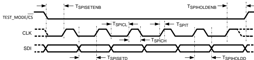
Figure 13. SPI Timing
