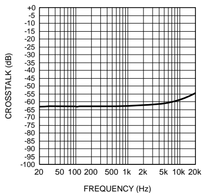
Headphone Crosstalk vs Frequency OCL 1.2V, 0dB AUX, 32Ω
