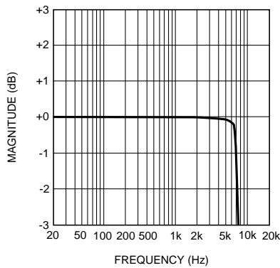
Stereo DAC Frequency Response f_S = 24kHz
