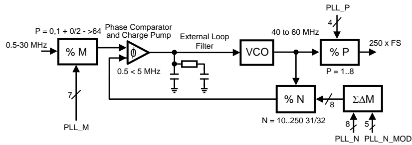
Figure 15. PLL Overview
