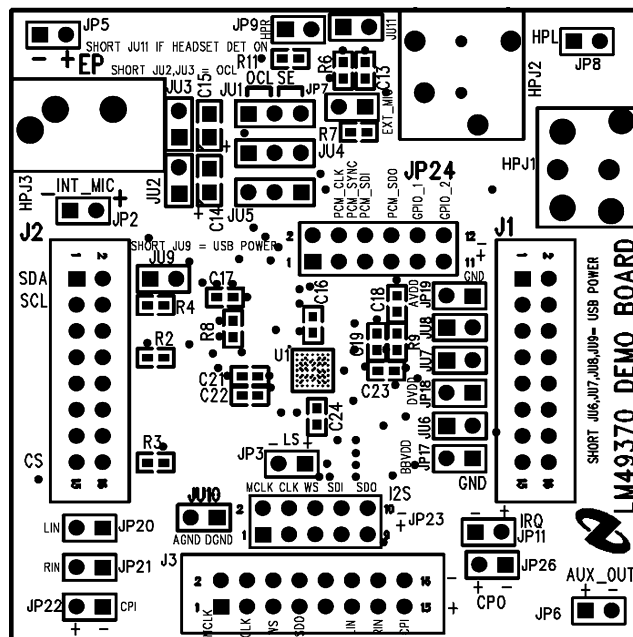
Figure 28. Top Silkscreen
