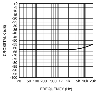
Headphone Crosstalk vs Frequency OCL 1.5V, 0dB AUX, 32Ω
