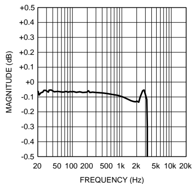
MONO ADC Frequency Response Zoom f_s = 8kHz , 6dB MIC
