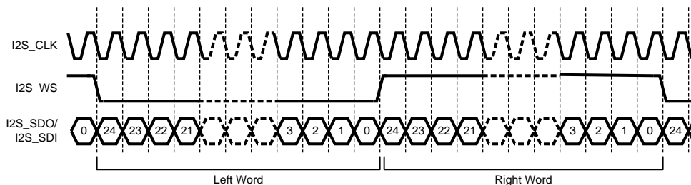
Figure 21. I 2 S Serial Data Format (Left Justified)
