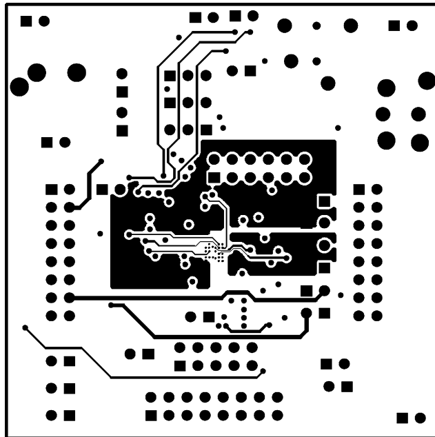
Figure 31. Mid Layer 2
