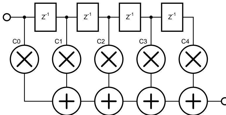
Figure 25. FIR Consumption Filter Taps
