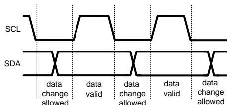
Figure 5. I 2 C Signals: Data Validity
