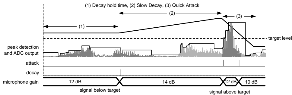
Figure 16. AGC Operation Example
