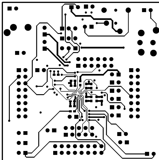
Figure 32. Bottom Layer
