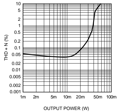
Headphone THD+N vs Output Power AV_{DD} = 3.3V, SE, 0dB AUX f_{OUT} = 1kHz, 32\Omega
