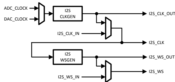
Figure 19. I2S Audio Port CLOCK/SYNC Options
