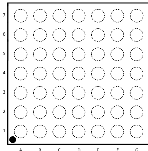
49 Bump micro SMDxt
