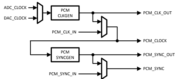
Figure 23. PCM Audio Port CLOCK/SYNC Options
