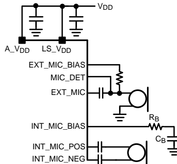
Figure 26. Schematic for MEMs Microphones
