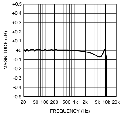
MONO ADC Frequency Response Zoom f_s = 24kHz, 6dB MIC
