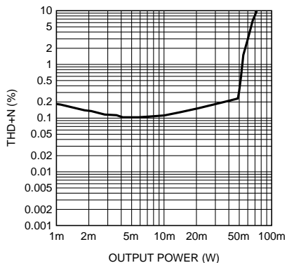
Headphone THD+N vs Output Power AV_{DD} = 5V , OCL 1.5V, 12dB DAC f_{OUT} = 1kHz , 16Ω
