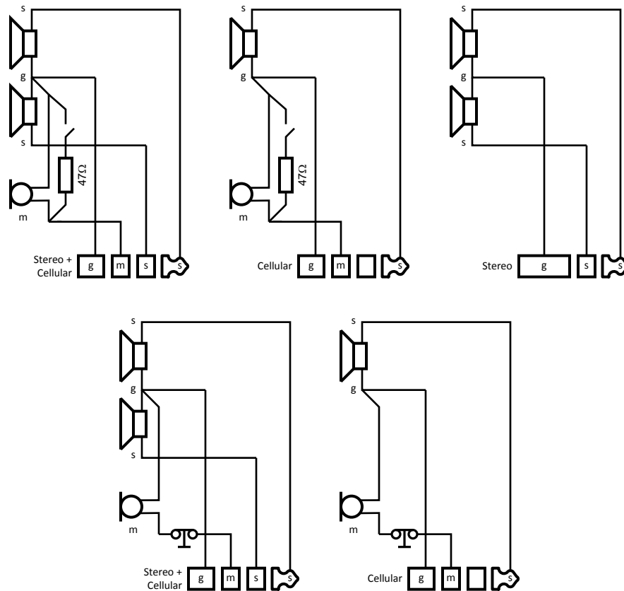
Figure 17. Headset Configurations Supported by the LM49370
