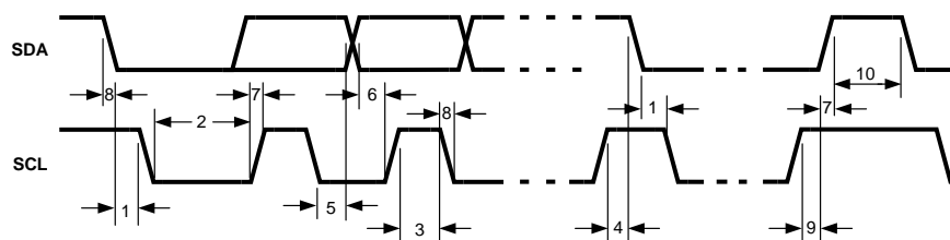
Figure 9. I 2 C Timing Diagram
