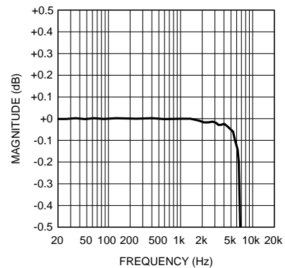
Stereo DAC Frequency Response Zoom f_S = 16kHz
