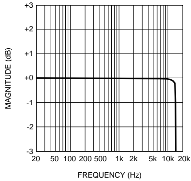
Stereo DAC Frequency Response f_s = 48kHz
