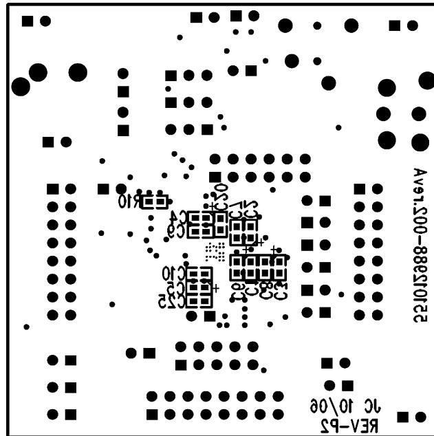
Figure 33. Bottom Silkscreen
