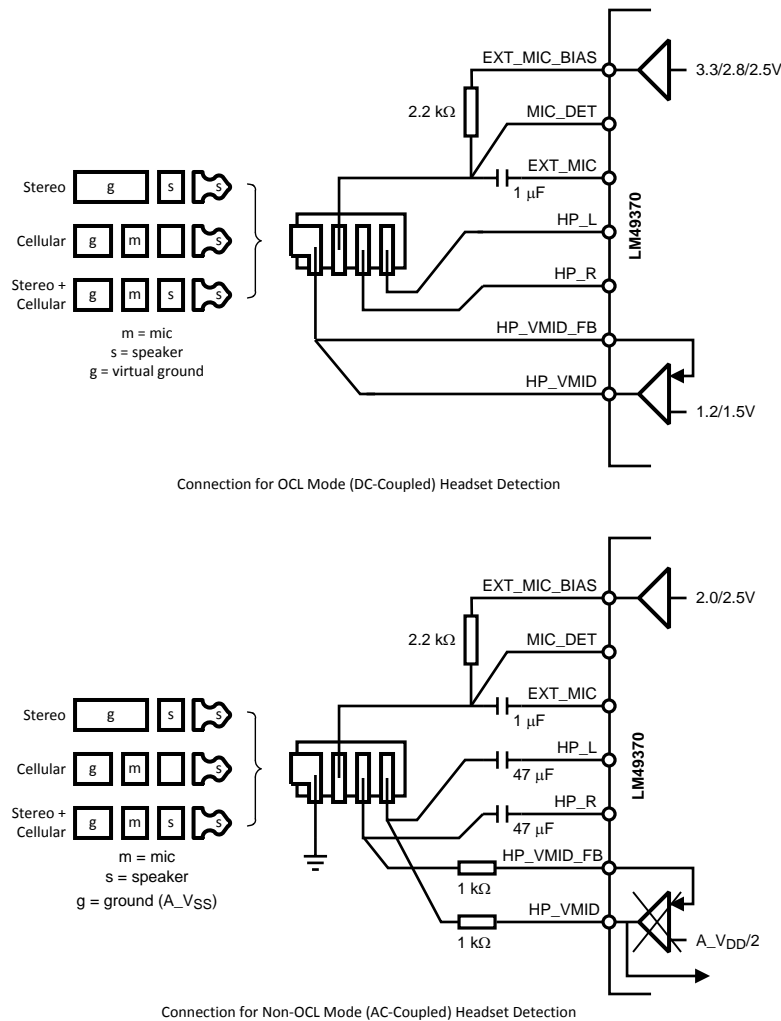
Figure 18. Connection of Headset Jack to LM49370 Depends on the Mode of the Headphone Amplifier.
