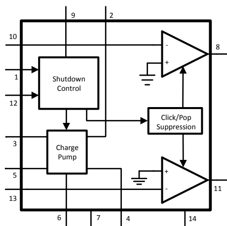
Figure 1. Circuit Block Diagram
