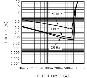
THD+N vs Output Power V_{DD} = 5V , 8\Omega R_L
