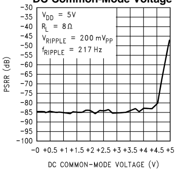
DC Common-Mode Voltage PSRR vs
