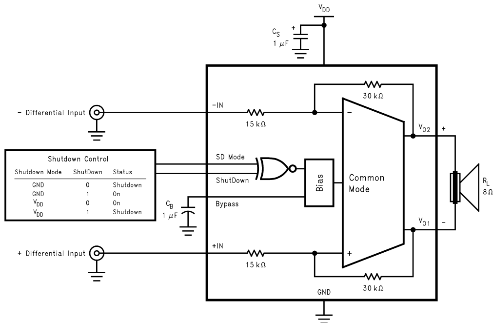
Figure 1. Typical Audio Amplifier Application Circuit
