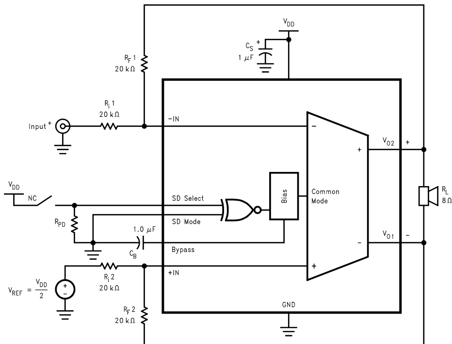
Figure 2. Single-Ended Input, "Shutdown-Low" Configuration
