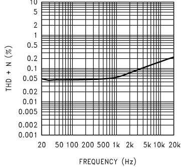
THD+N vs Frequency at V_{DD} = 3V , 4\Omega R_L , and PWR = 225mW
