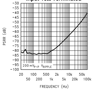
Power Supply Rejection Ratio (PSRR) at V_{DD} = 3V Input 10\Omega Terminated
