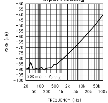
Power Supply Rejection Ratio (PSRR) at V_{DD} = 3V Input Floating
