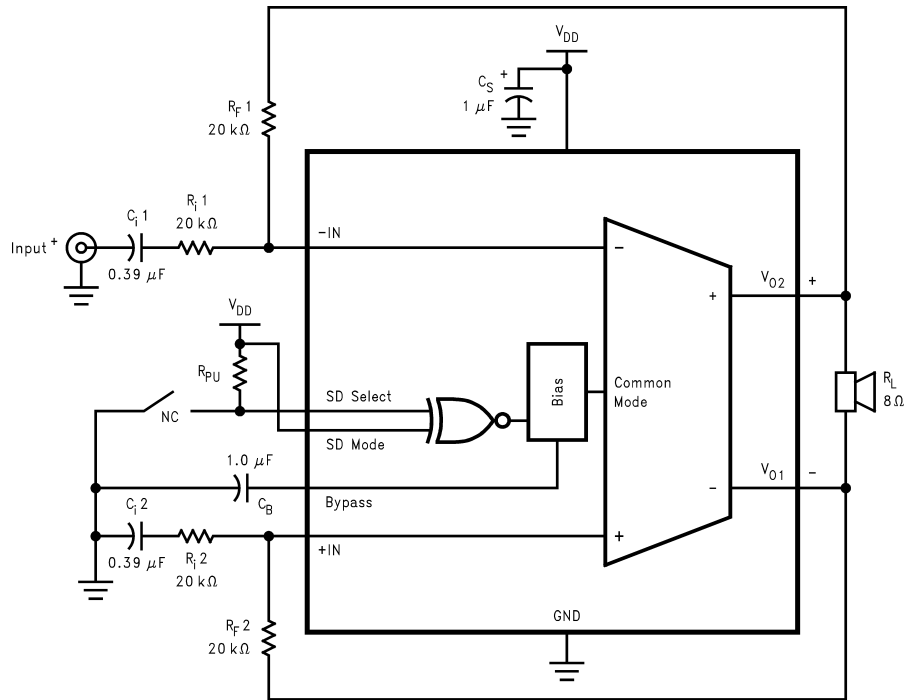
Figure 3. Single-Ended Input, "Shutdown-High" Configuration
