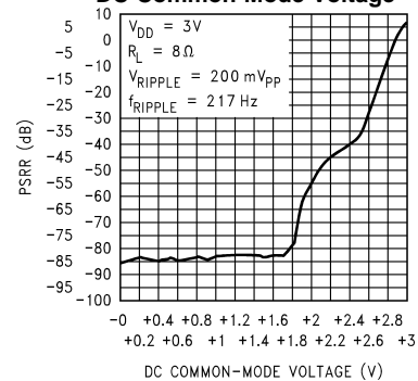
PSRR vs DC Common-Mode Voltage
