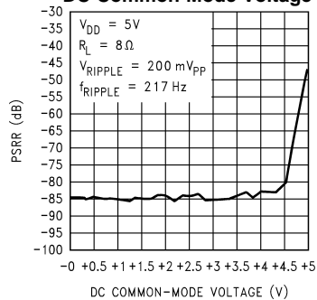
PSRR vs DC Common-Mode Voltage
