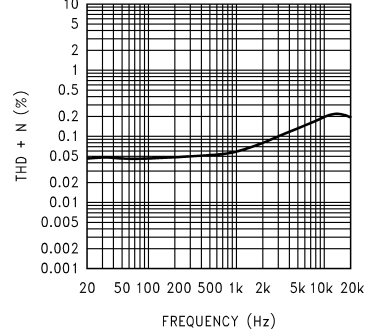
THD+N vs Frequency at V_{DD} = 2.6V , 8\Omega R_L , and PWR = 150mW
