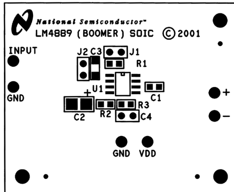
Figure 24. Silk Screen
