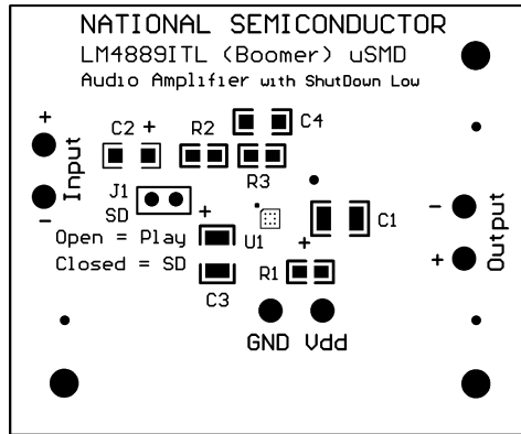
Figure 18. Silk Screen
