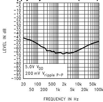
Figure 10. Input terminated with 10\Omega R
