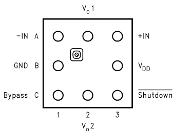
Figure 6. 8-Bump micro SMD
