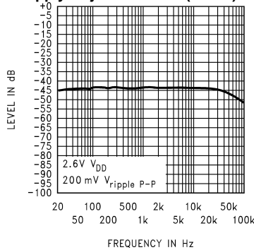
Figure 12. Input terminated with 10\Omega R
