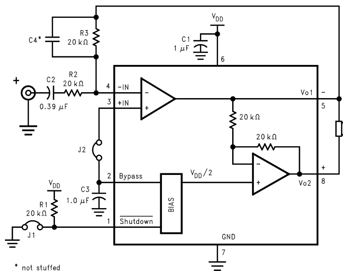
Figure 23. Reference Design Board
