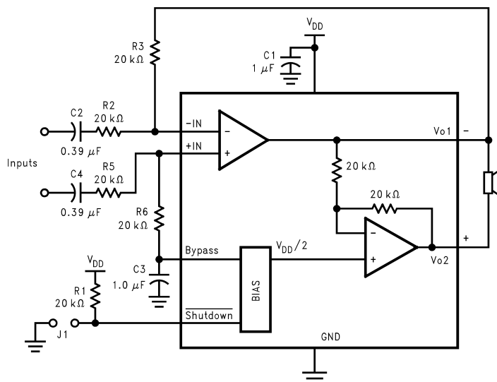
Figure 15. Differential Amplifier Configuration for LM4889
