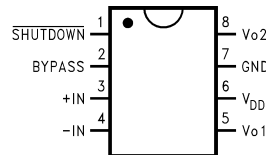
Figure 2. Small Outline (SO) Package
