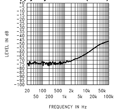
Figure 11. Input Floating
