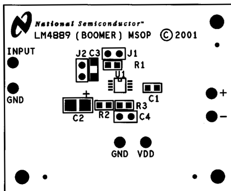
Figure 27. Silk Screen
