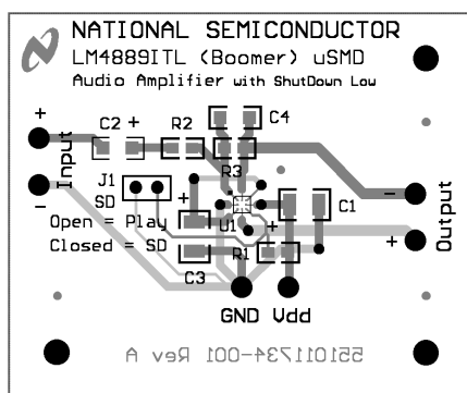
Figure 17. Composite View
