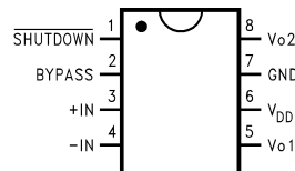
Figure 4. Mini Small Outline (MSOP) Package
