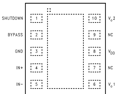
Figure 8. LLP Package
