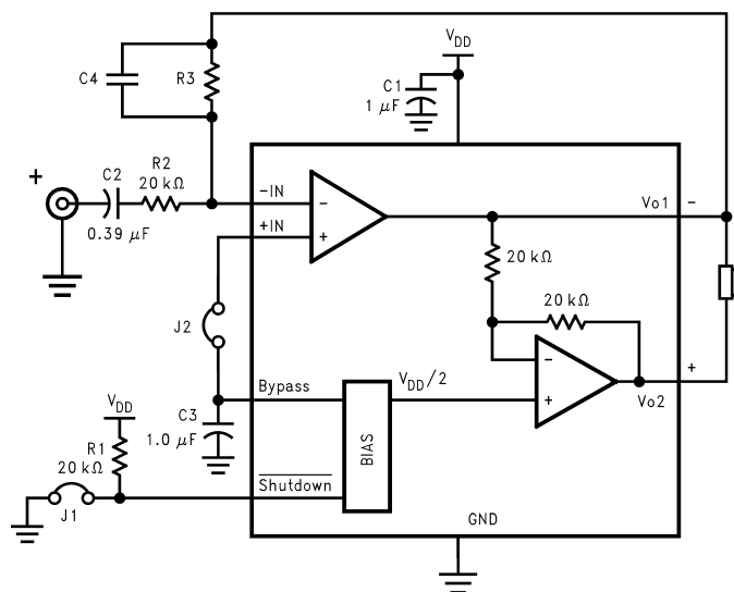
Figure 14. Higher Gain Audio Amplifier
