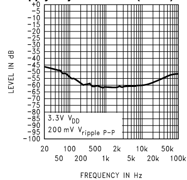
Figure 13. Input terminated with 10\Omega R
