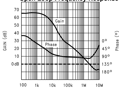
Open Loop Frequency Response
