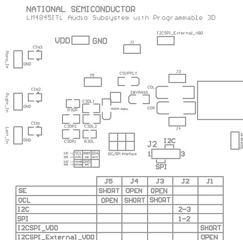
Figure 72. Top Overlay
