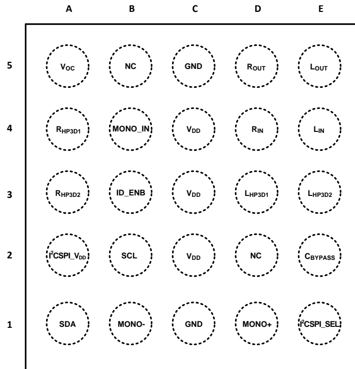
Figure 3. 25-Bump DSBGA Top View
