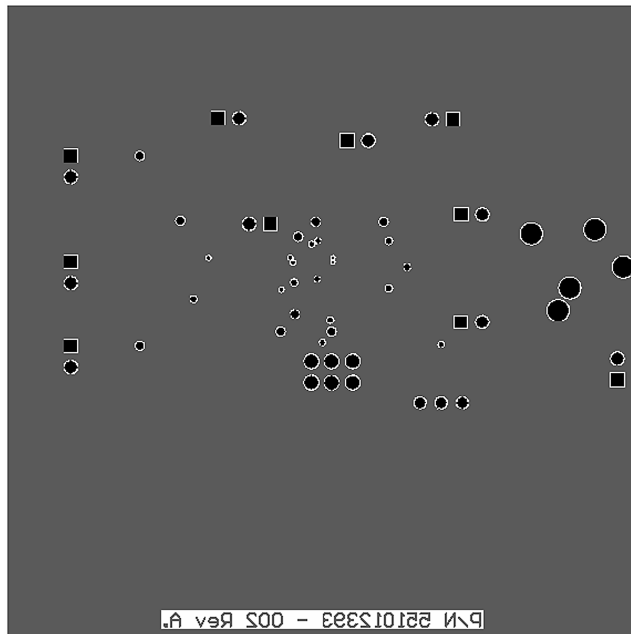
Figure 74. Bottom Layer
