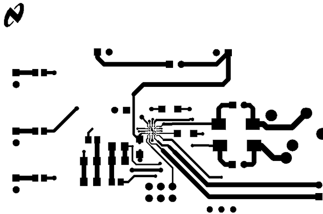
Figure 74. Bottom Layer
