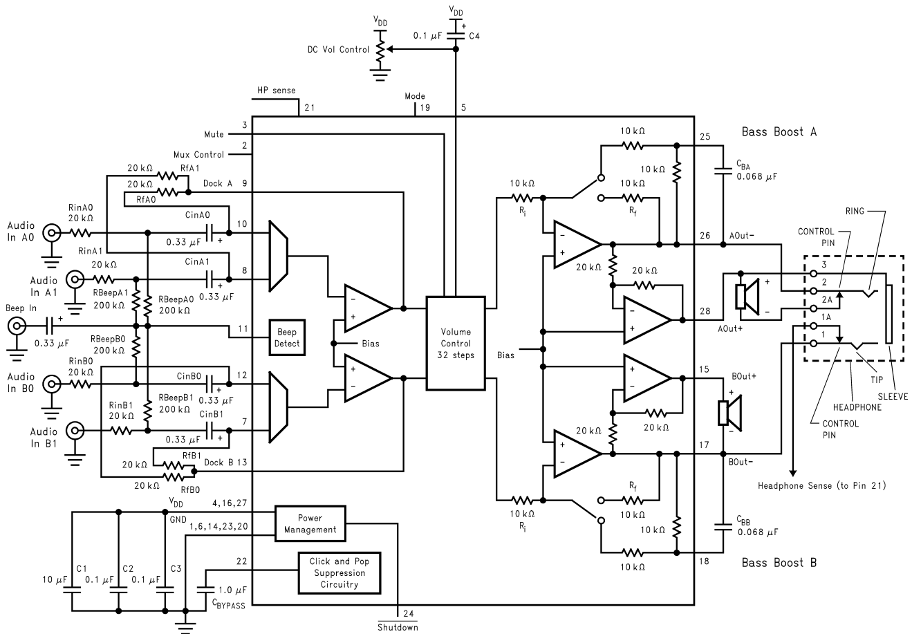
Figure 2. Typical Application Circuit ( MT & MH pinout )
