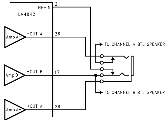
Figure 5. Headphone Sensing Circuit
