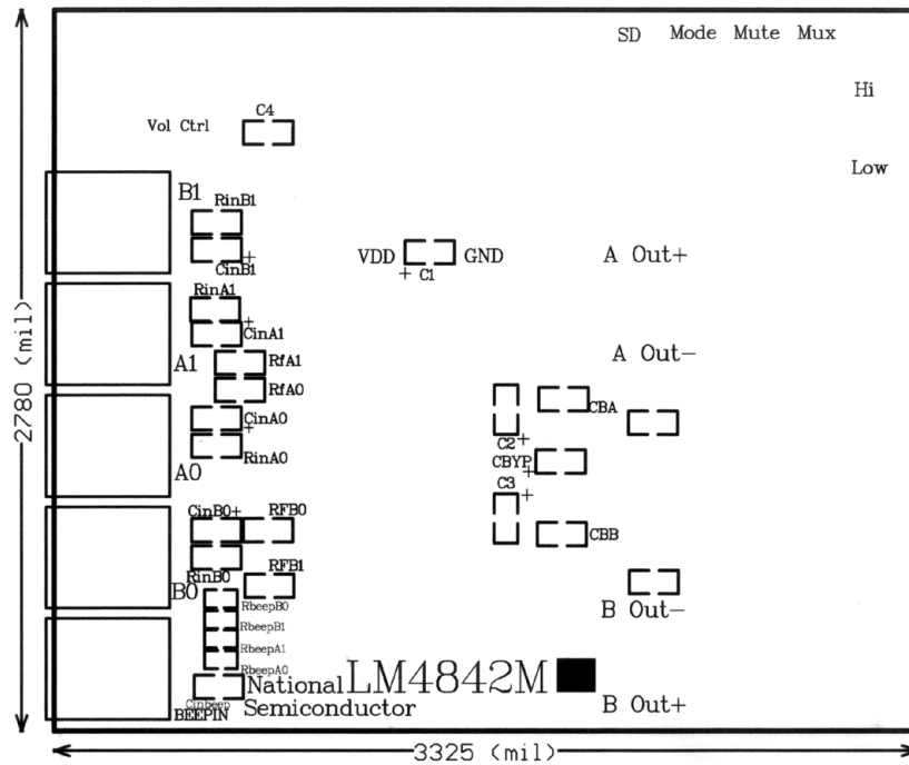
Figure 7. Top Layer SilkScreen - ( Not to Scale )
