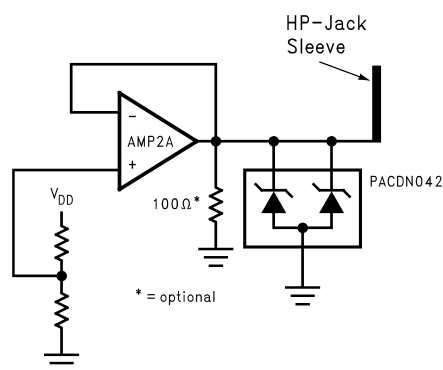
Figure 6. The PACDN042 provides additional ESD protection beyond the 6500V shown in the Absolute Maximum Ratings for the AMP2A output
