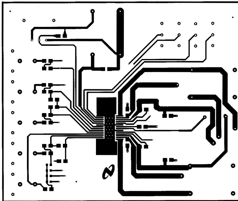
Figure 8. Top Layer - ( Not to Scale )
