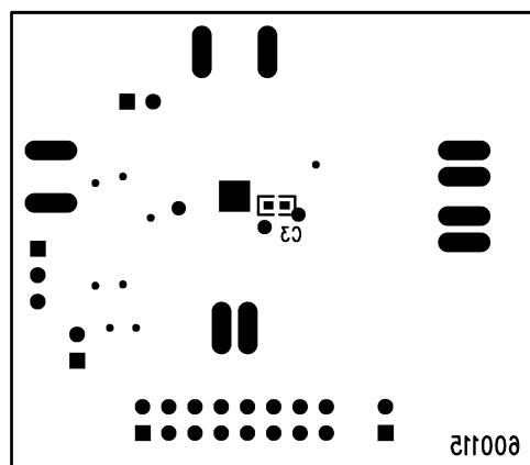
Figure 23. Bottom Silkscreen
