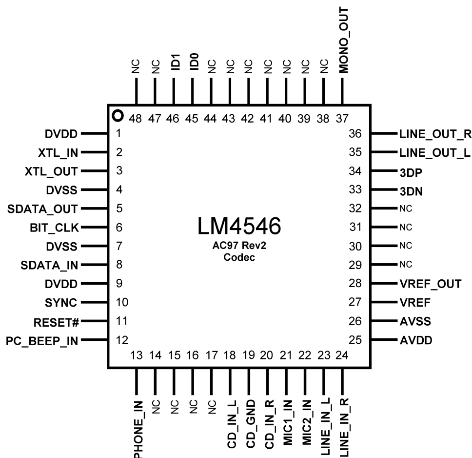
Figure 8. Top View Order Number LM4546VH See NS Package Number VBH48A
