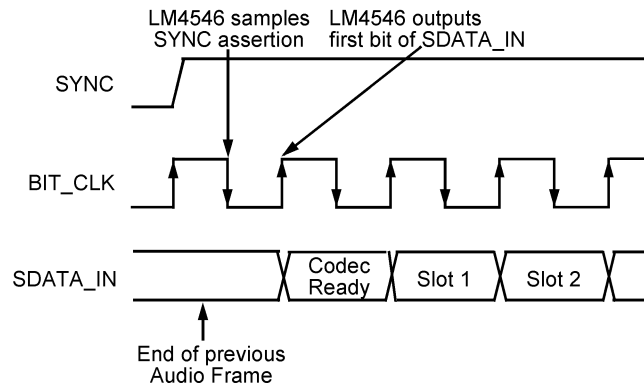
Figure 13. Start of Audio Input Frame
