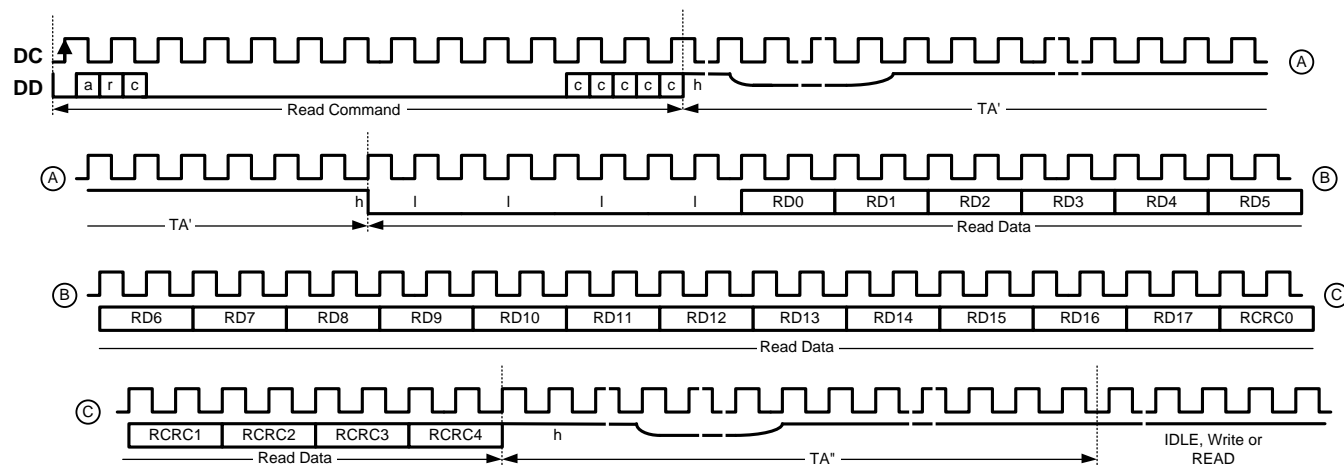
Figure 10. READ Transaction
