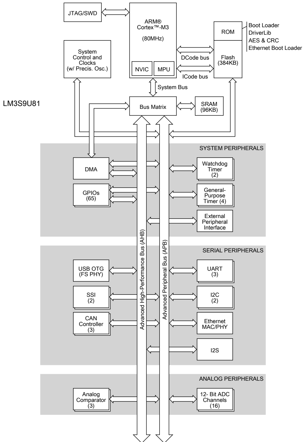
Figure 1-1. Stellaris LM3S9U81 Microcontroller High-Level Block Diagram
