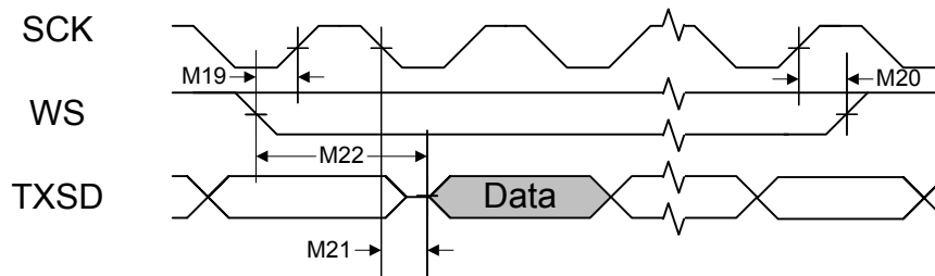
Figure 26-20. I 2 S Slave Mode Transmit Timing
