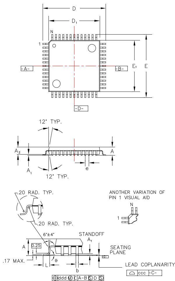
Figure C-1. Stellaris LM3S9DN6 100-Pin LQFP Package Dimensions
