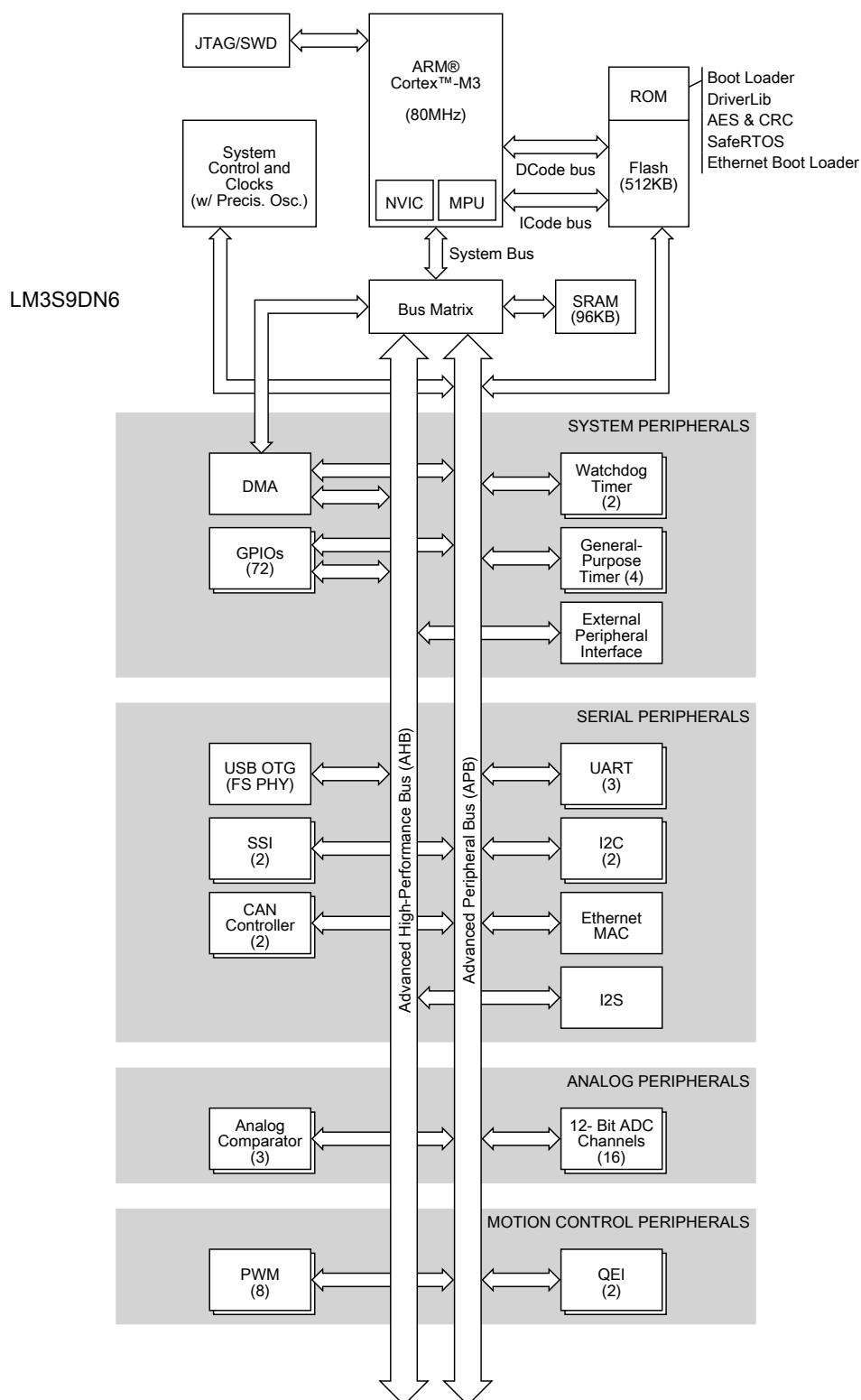
Figure 1-1. Stellaris LM3S9DN6 Microcontroller High-Level Block Diagram
