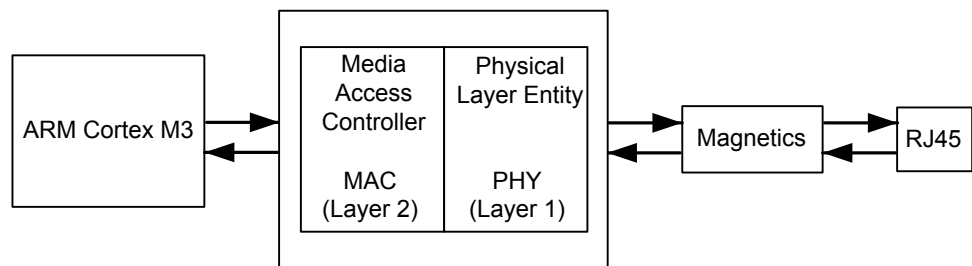
Figure 12-1. Ethernet Controller
