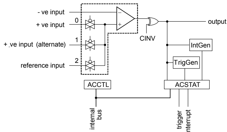
Figure 13-2. Structure of Comparator Unit
