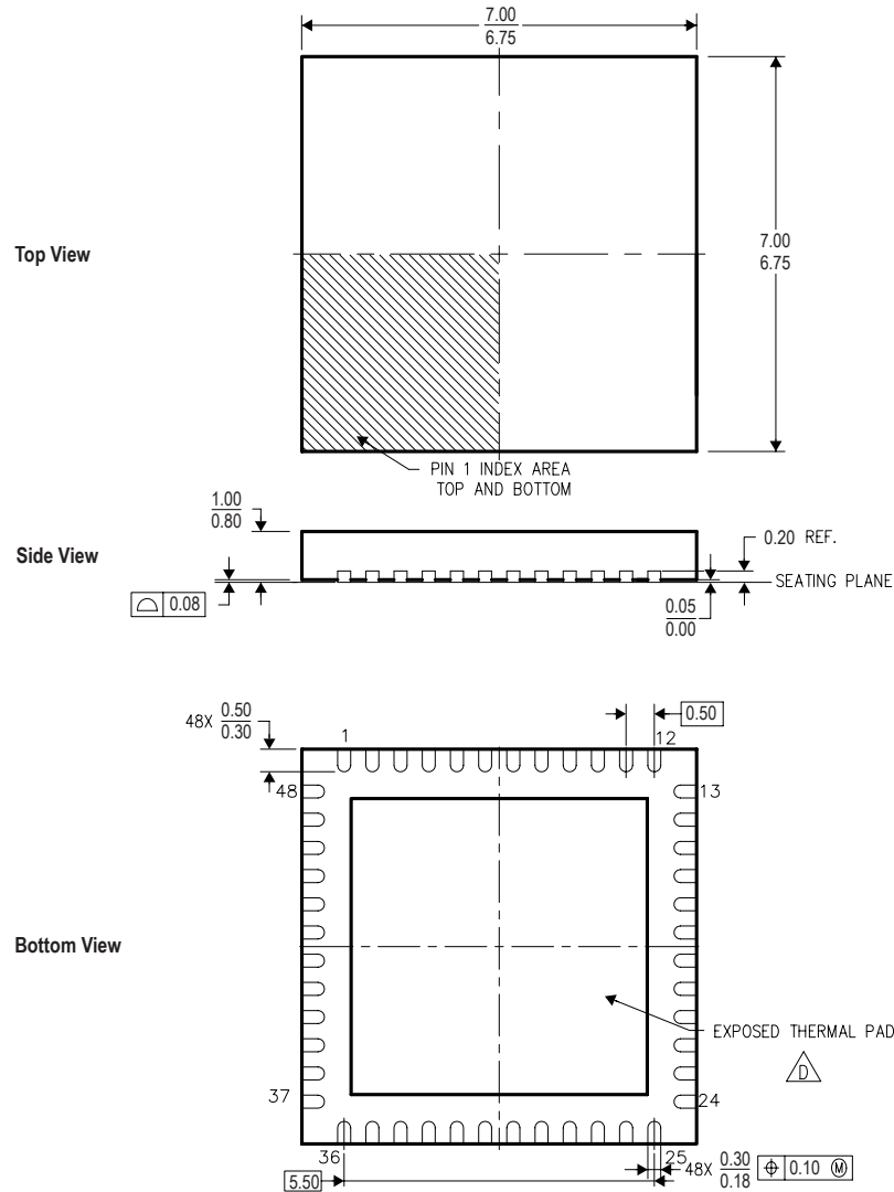
Figure D-4. Stellaris LM3S611 48-Pin QFN Package
