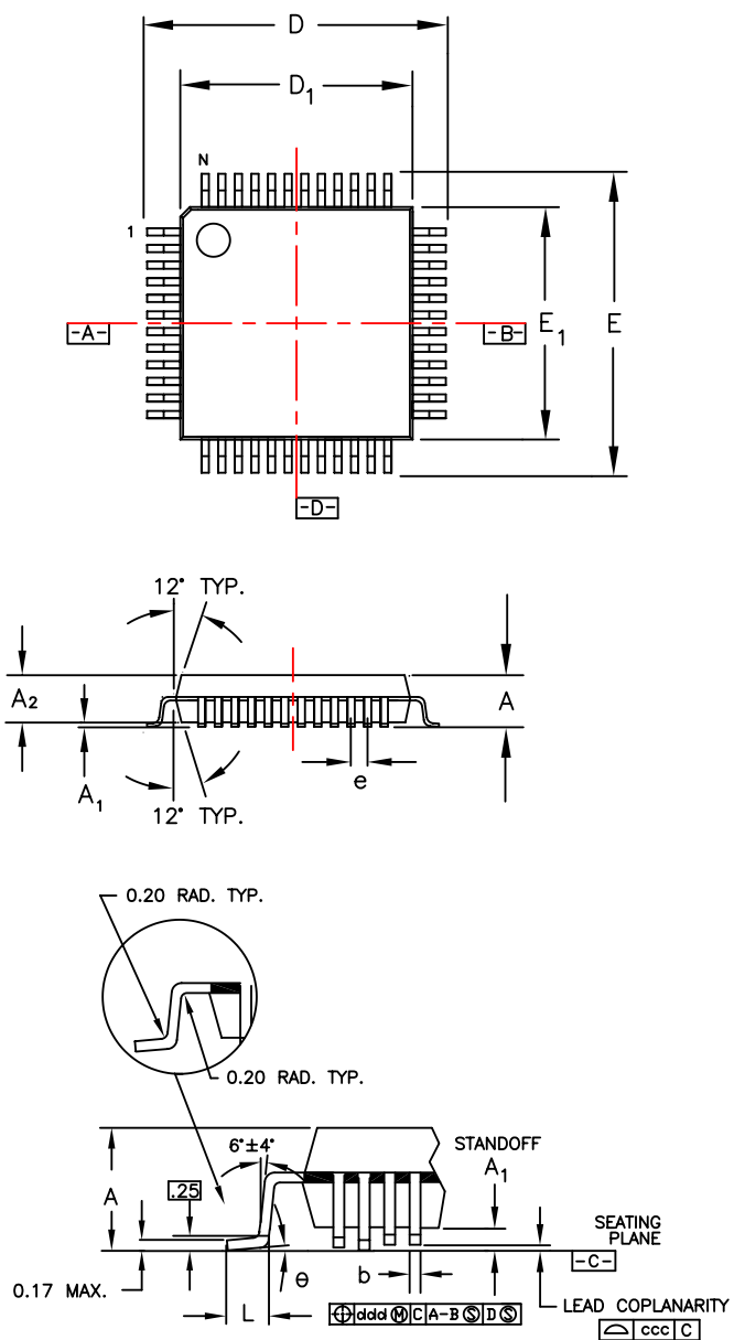
Figure D-1. Stellaris LM3S601 48-Pin LQFP Package
