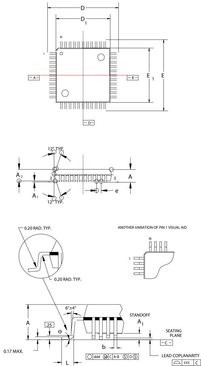
Figure E-1. Stellaris LM3S2776 64-Pin LQFP Package
