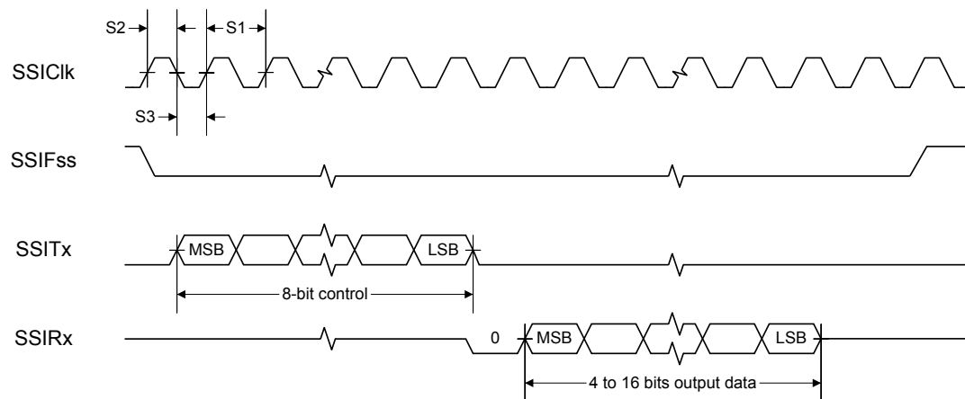
Figure 19-11. SSI Timing for MICROWIRE Frame Format (FRF=10), Single Transfer
