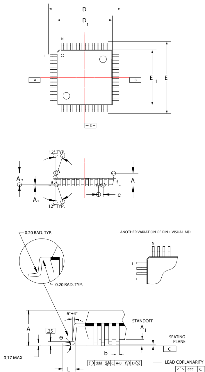
Figure C-1. Stellaris LM3S1R26 64-Pin LQFP Package
