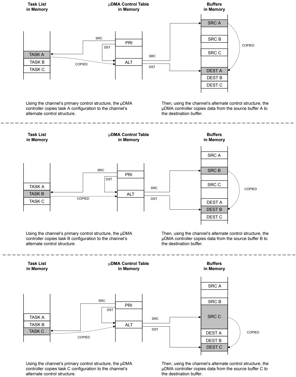
Figure 7-4. Memory Scatter-Gather, \mu DMA Copy Sequence
