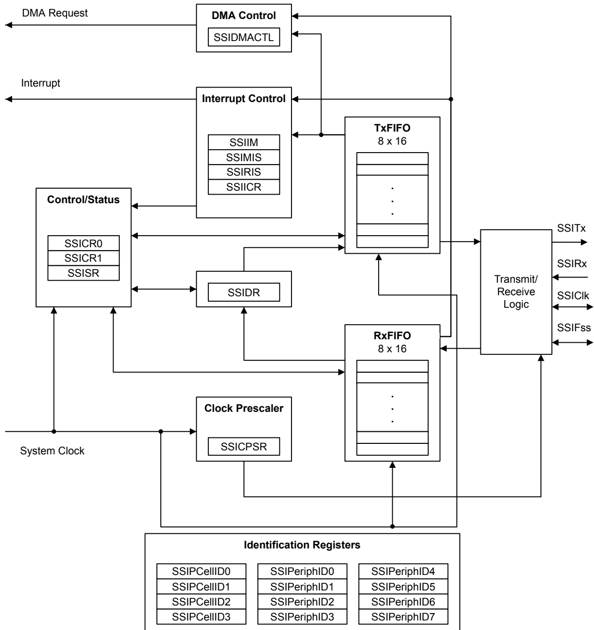
Figure 13-1. SSI Module Block Diagram
