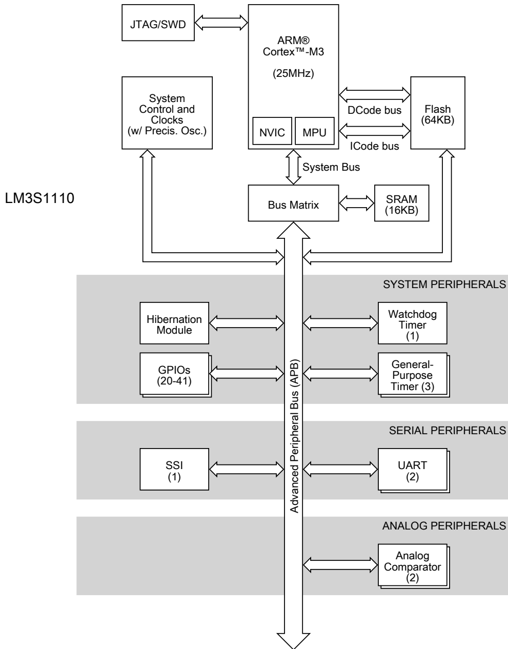
Figure 1-1. Stellaris LM3S1110 Microcontroller High-Level Block Diagram
