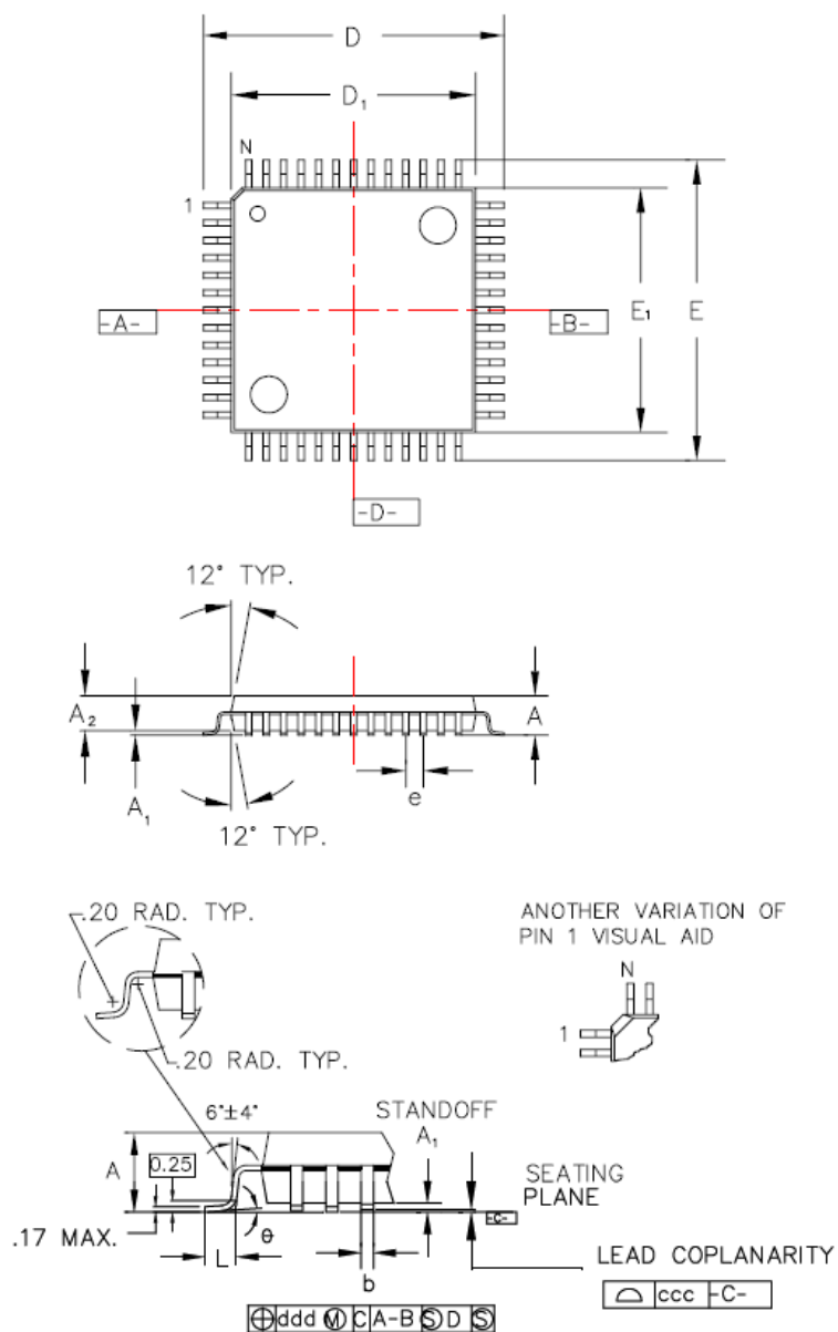
Figure D-1. Stellaris LM3S1110 100-Pin LQFP Package Dimensions
