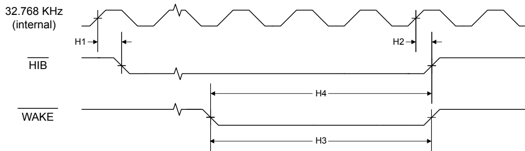
Figure 17-10. Hibernation Module Timing
