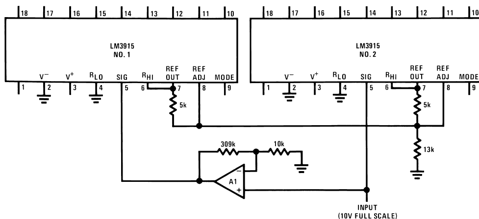
Figure 22. Improved Circuit for 60 dB Display
