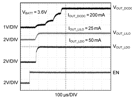
Figure 23. Startup Sequence, V EN_DCDC = V EN_LILO = V EN_LDO = V BATT
