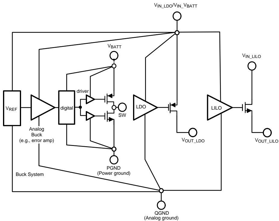
Figure 2. Functional Diagram (Always Connect V IN_LDO to V BATT )
