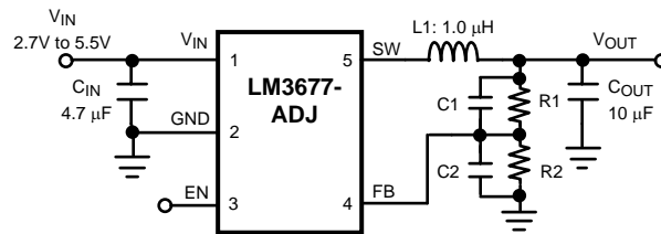
Figure 3. Typical Application Circuit - ADJ. Version
