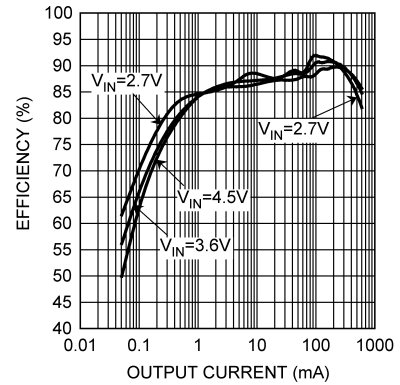
Figure 2. Efficiency vs. Output Current (V OUT = 1.8V)
