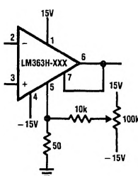
b. Output Offset Adj. for 8-Pin Package
