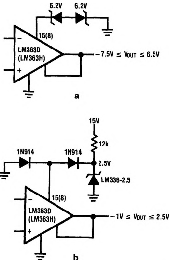
FIGURE 7. Output Clamp
