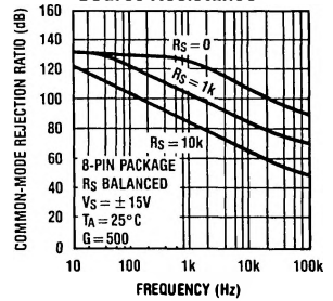
CMRR with Balanced Source Resistance
