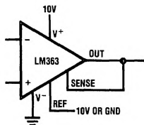
c. Single Supply, Unipolar Output
