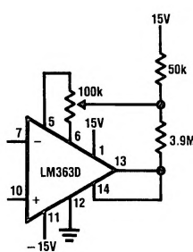
b. Gain
