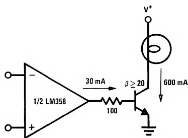
Lamp Driver
