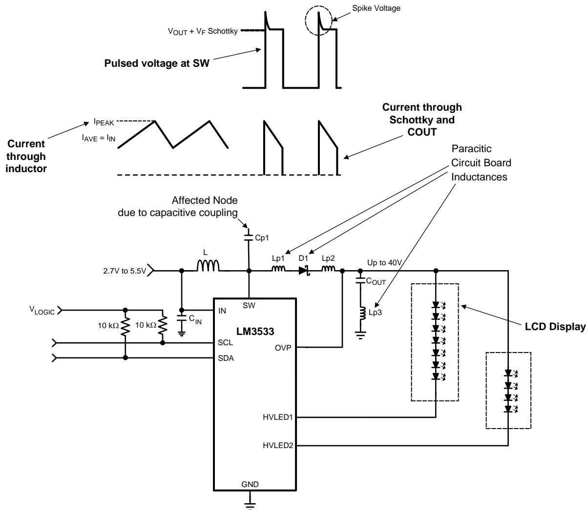
Figure 19. LM3533's Inductive Boost Converter Showing Pulsed Voltage at SW (High dV/dt) and Current Through Schottky and COUT (High dI/dt)
