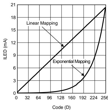
Figure 6. LED Current Mapping Modes
