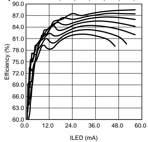
Efficiency vs ILED L = 10\mu H, V_{IN} = 3.6V, f_{SW} = 1MHz Top to Bottom: 2x4, 2x5, 2x6, 2x7, 2x8, 2x9, 2x10 (LEDs)
