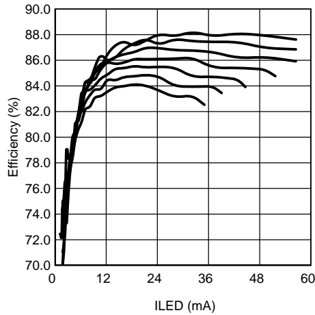
Efficiency vs ILED L = 4.7\mu H, V_{IN} = 3.6V, f_{SW} = 1MHz Top to Bottom: 2x4, 2x5, 2x6, 2x7, 2x8, 2x9, 2x10 (LEDs)
