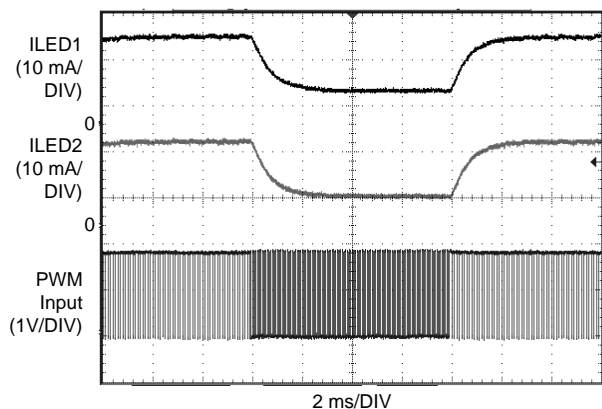
Response to Step Change in PWM Input Duty Cycle ( D = 30\% to 90\% , f_{PWM} = 10kHz , I_{LED\_FULL\ SCALE} = 20.2mA )
