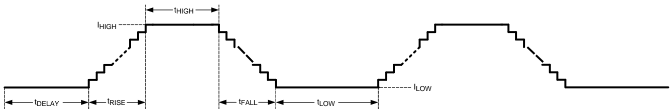
Figure 18. Pattern Generator Timing
