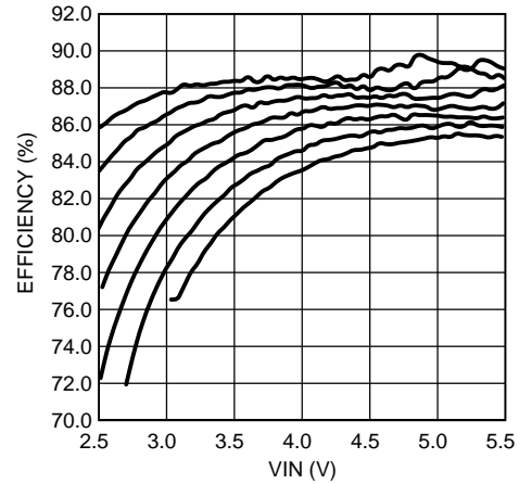
Efficiency vs VIN, Single String L = 10\mu H , 20mA/string , f_{SW} = 1MHz Top to Bottom: 1x4, 1x5, 1x6, 1x7, 1x8, 1x9, 1x10 (LEDs)
