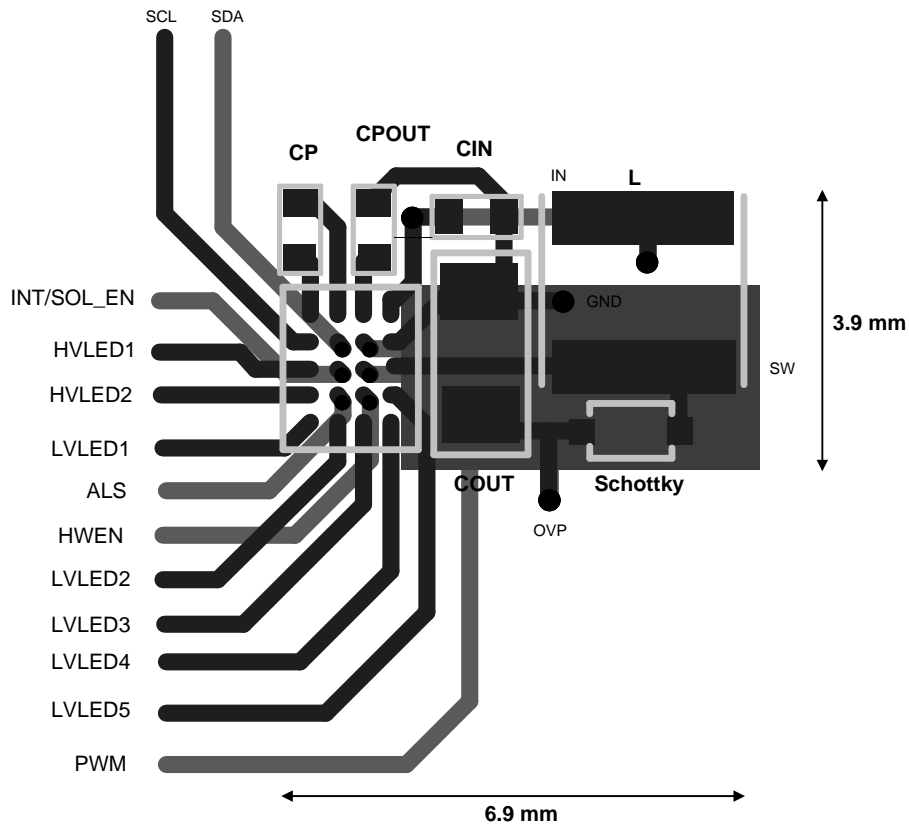
Figure 21. LM3533 Example Layout
