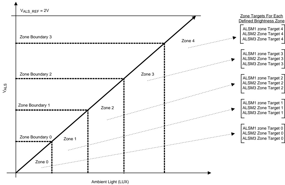
Figure 8. ALS Brightness Zone to Backlight Current Mapping
