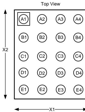
Figure 1. 20-Bump DSBGA Package (Top View) Package YFQ0020GAA
