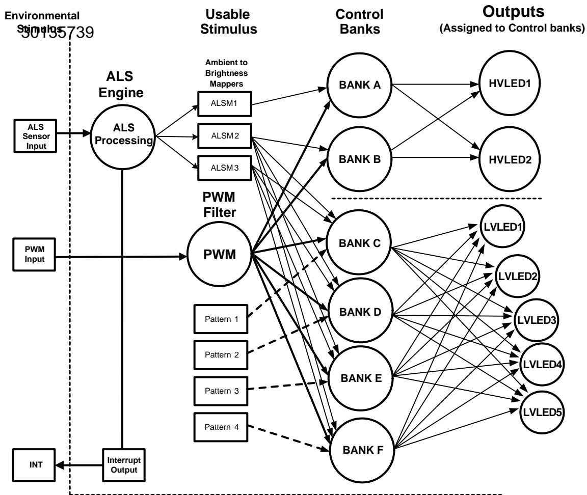
Figure 4. Functional Control Diagram
