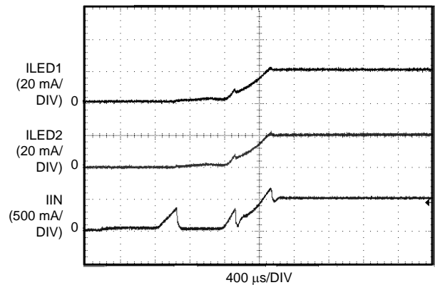
Startup Response (VIN = 3.6V, 2x8 LEDs, 20mA/string)
