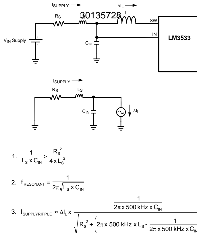
Figure 20. Input RLC Network
