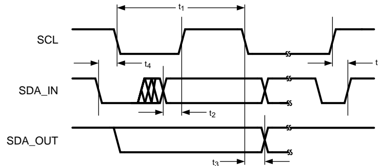
Figure 2. I 2 C-Compatible Interface Timing
