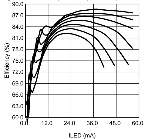
Efficiency vs ILED L = 22μH, VIN = 3.6V, fSW = 1MHz Top to Bottom: 2x4, 2x5, 2x6, 2x7, 2x8, 2x9, 2x10 (LEDs)
