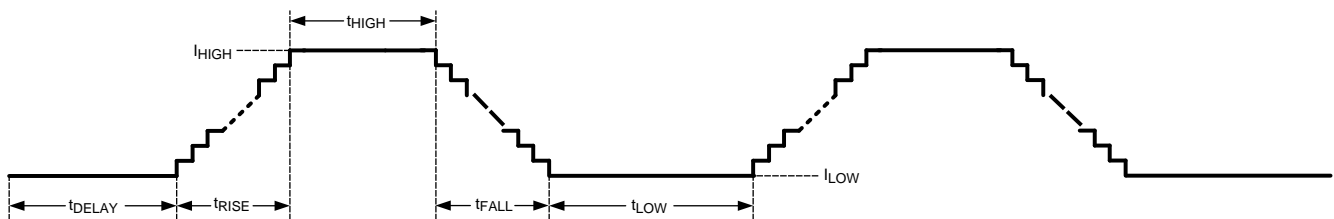
Figure 15. Pattern Generator Timing
