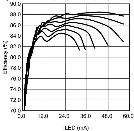
Efficiency vs ILED L = 22μH, VIN = 3.6V, fSW = 500kHz Top to Bottom: 2x4, 2x5, 2x6, 2x7, 2x8, 2x9, 2x10 (LEDs)
